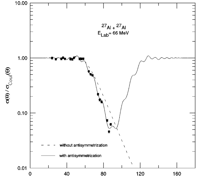
FIG. 2. Comparison of the calculation of the elastic angular distribution with and without effect of the antisymmetrization of the wave function, normalized at the cross section calculated with a pure Coulomb potential [ \sigma_{\text{Coul}}(\theta) ].
