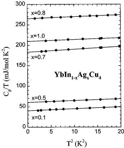
FIG. 1. The low-temperature specific heat C_p(T) of \text{YbIn}_{1-x}\text{Ag}_x\text{Cu}_4 plotted as C_p(T)/T versus the square of the temperature for several values of alloy concentration x . The solid lines are fits to the functional form C_p(T) = \gamma T + \delta T^3 .
