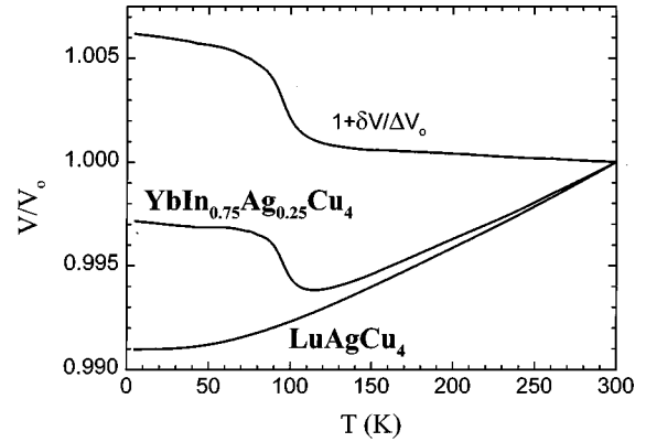
FIG. 7. The cell volume V(T)/V_0 (where V_0 is the room-temperature volume) for \text{YbIn}_{0.75}\text{Ag}_{0.25}\text{Cu}_4 and \text{LuAgCu}_4 plotted versus the temperature. The anomalous contribution to the cell volume \delta V(T)/V_0 is the difference between these two curves.
