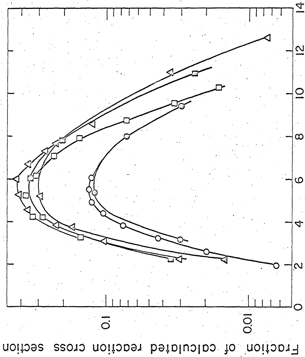
Fig. 5 Available energy per emitted neutron (Mev)
