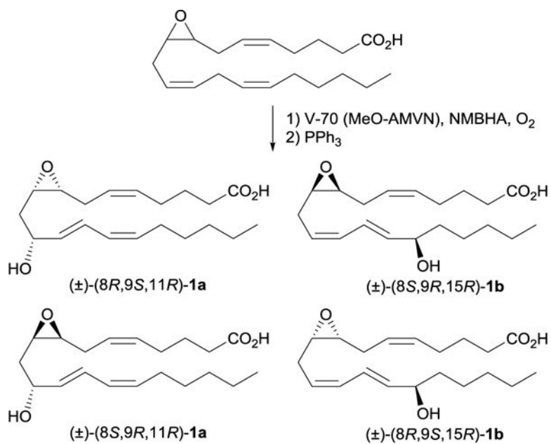
Scheme 1. Radical biomimetic oxidation of (±)-8,9-EET produce all 8 isomeric EHETs
