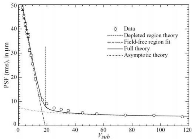
Fig. 4. The measured rms diffusion (data points) as a function of the substrate bias voltage. The data are for a 193 \mu\text{m} thick high voltage CCD, and at the highest voltage, the diffusion is lower than the 4 \mu\text{m} SNAP design goal. The field-free region line is the theoretical fit for operation below full depletion, the depleted region line is the theoretical prediction for over-depleted operation, and the full theory line is the convolution of both.
