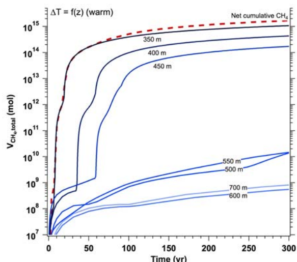
Figure 8. Cumulative local fluxes of methane in gaseous and aqueous phases, V_{CH_4, tot} , for a warm scenario ( \Delta T = 1 °C - 5 °C/100 yr), plus the total basin-wide net flux (red line).
