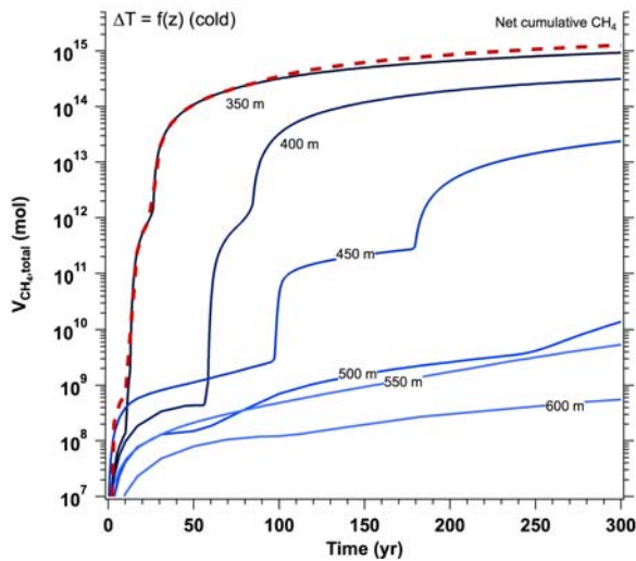
Figure 9. Cumulative local fluxes of methane in gaseous and aqueous phases, V_{\text{CH}_4,\text{tot}} , for a cold scenario ( \Delta T = 0^\circ\text{C} - 3^\circ\text{C}/100 yr), plus the total basin-wide net flux (red line).
