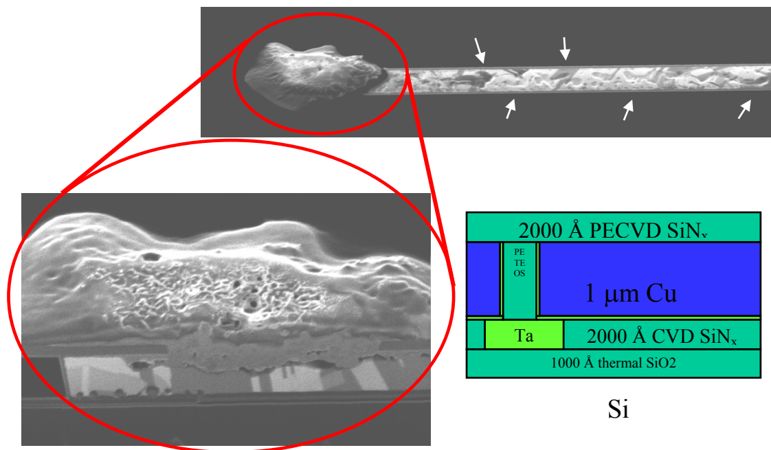
FIGURE 1. Electromigration damage in a Blech type, 2 micron wide, Cu damascene line, the lower right part shows a schematic of the crosssection visible in the lower left part, white arrows indicate surface voids. The hillock on the top left has cracked the passivation at test temperature and has consequently oxidized.
