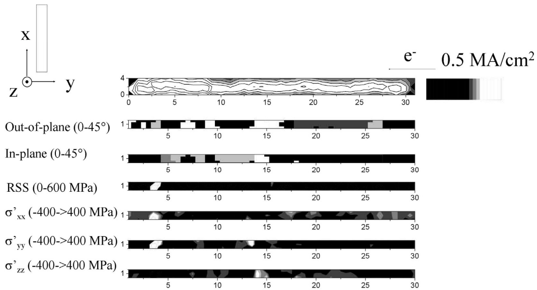
FIGURE 4. Orientation and stress maps of a 0.8 μm wide, 30 μm long damascene Blech segment during an electromigration test. In the out of plane map black areas are (111) oriented, white are (115) oriented and grey areas are (5 7 13) oriented. The range of the black to white contrast is indicated in brackets beside the maps.
