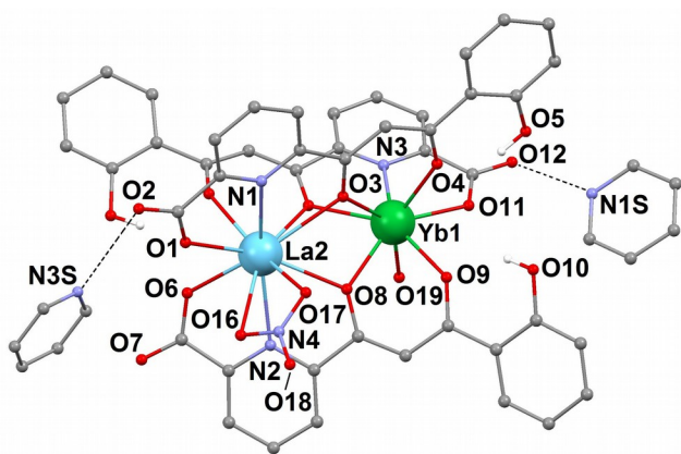
Figure 4. Molecular structure of the complex cation of (Hpy) 2 [LaYb(HL) 3 (NO 3 )(H 2 O)](NO 3 ) ( 5 ), emphasizing the hydrogen bonds established between two of its -COO - groups and two pyridinium cations. All heteroatoms are labelled, C atoms are in grey and only H atoms of the phenol groups shown in white.
