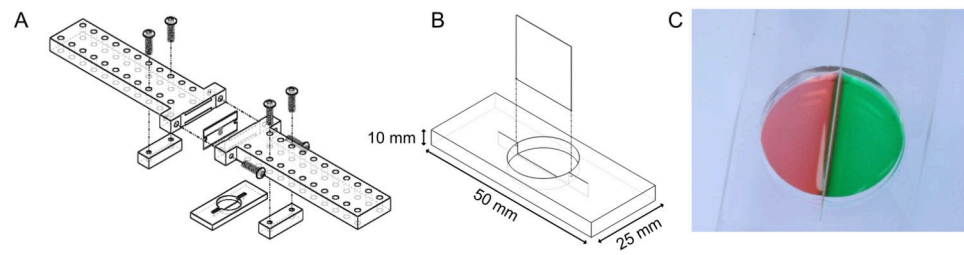
Figure 2. Reconfigurable elastic substrate device. (A) Schematic of cutting apparatus. (B) Device consists of a molded elastic well with a slit extending partially through the well bottom. (C) The device seals around an inserted coverslip to form two isolated chambers.
