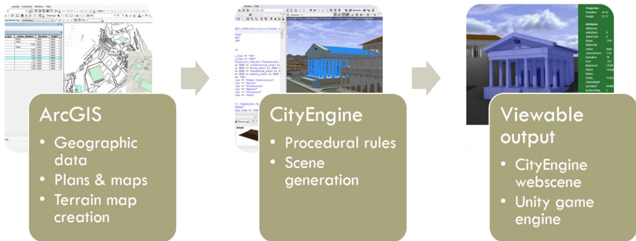
Fig. 15 Workflow overview
