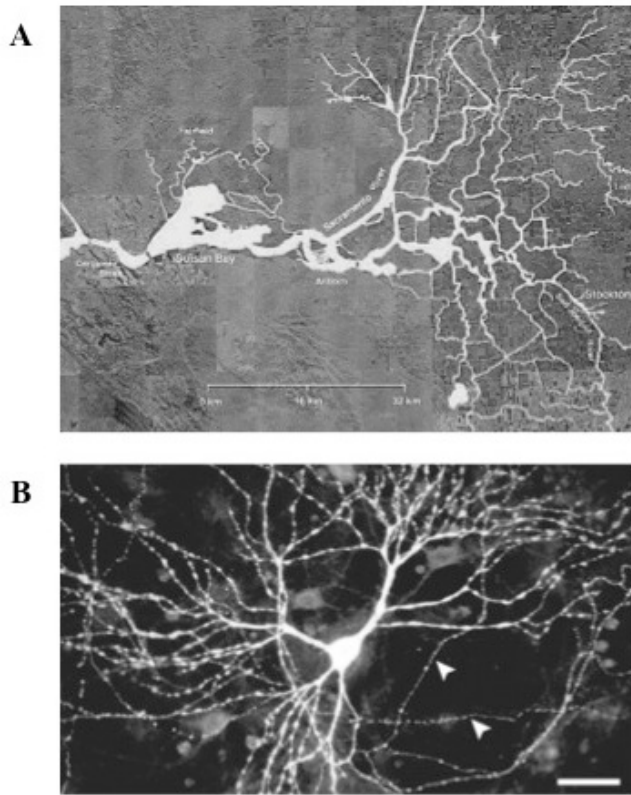
Figure 2: Increased energy flow results in increased speed of flow. (A) River flow of California’s Sacramento-San Joaquin River delta (modified from Trump, 2004). (B) Expression of TRPV1, a receptor protein, in cultured hippocampal neurons (Zemelman et al., 2003). The hippocampus and receptor proteins such as TRPV1 are associated with memory formation in the brain (e.g., Gibson et al. 2008).
