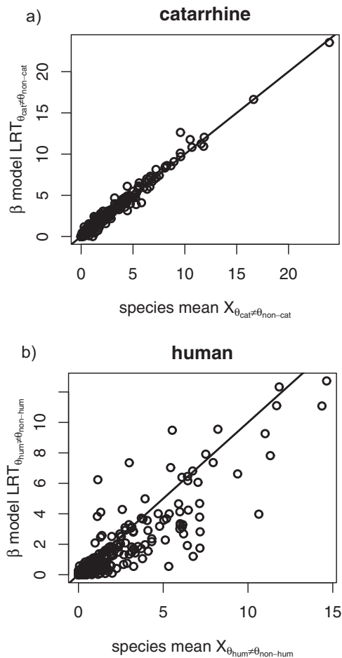
FIGURE 5. Each plot shows (a) LRT_{\theta_{cat} \neq \theta_{non-cat}} and (b) LRT_{\theta_{hum} \neq \theta_{non-hum}} calculated using the EVE model ( y -axes) and SM model ( x -axes) as implemented in this analysis. The line indicates x = y .
