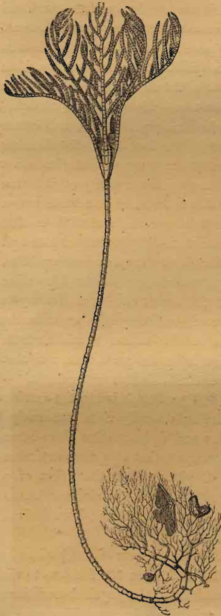
FIG. 17.— Rhizocrinus lofotensis , M. Sars.
