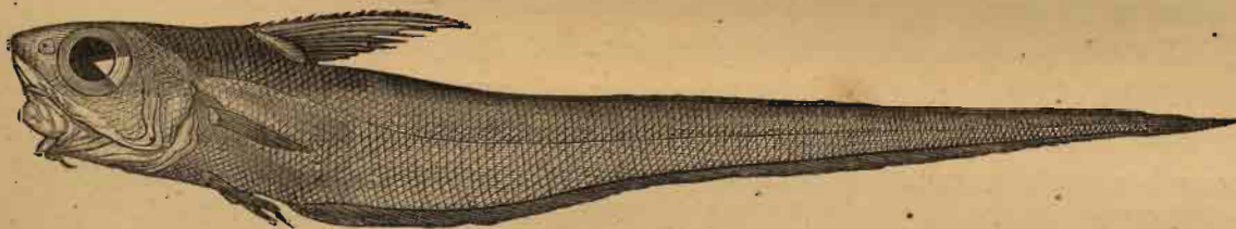
FIG. 24.— Ceryphæoides . A deep-sea fish belonging to the Macrurida.
