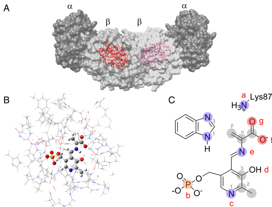
Fig. 4. Cluster model of the E(A-A) active site. (A) X-ray crystal structure of the TS \alpha_2\beta_2 heterodimer with the \beta -subunit active site highlighted in red. (B) Cluster model of the active site for first-principles geometry optimization and chemical shift calculations with protein side chains displayed in wireframe and cofactor and substrate in ball and stick. (C) Protonation sites on or near the cofactor/substrate complex: [a] the \beta Lys87 side chain, [b] the PLP phosphate group, [c] the PLP pyridine ring nitrogen, [d] the PLP phenolic oxygen, [e] the Schiff-base nitrogen, and [f/g] the substrate carboxylate. Shaded nuclei indicate sites for which experimental NMR chemical shifts are reported.
