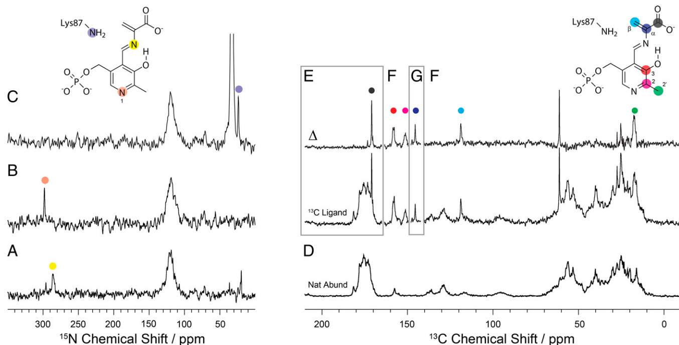
Fig. 3. ^{15}\text{N} and ^{13}\text{C} CPMAS SSNMR spectra of microcrystalline TS E(A-A) prepared with the following isotopic labeling: (A) ^{15}\text{N} -labeled on the substrate L-Ser; (B) ^{15}\text{N} -enriched on the PLP cofactor; (C) ^{15}\text{N} -enriched at protein lysine side-chain \epsilon -amino groups; (D) natural abundance isotopomer concentration; (E) ^{13}\text{C} -labeled at C' of the L-Ser substrate; (F) ^{13}\text{C} , ^{15}\text{N} -enriched on the PLP cofactor and C' of the substrate L-Ser; and (G) ^{13}\text{C} -labeled at C' of the substrate L-Ser. The top spectra in (E–G) are formed as the difference between the E(A-A) spectra with various cofactor/ligand isotopic labels and the same spectra acquired at natural abundance, emphasizing the resonances for the specific site labels. The large peak at 63.1 ppm is from free serine. Spectra acquired at 9.4 T, -10^\circ\text{C} , and 8 kHz MAS as described in Materials and Methods .
