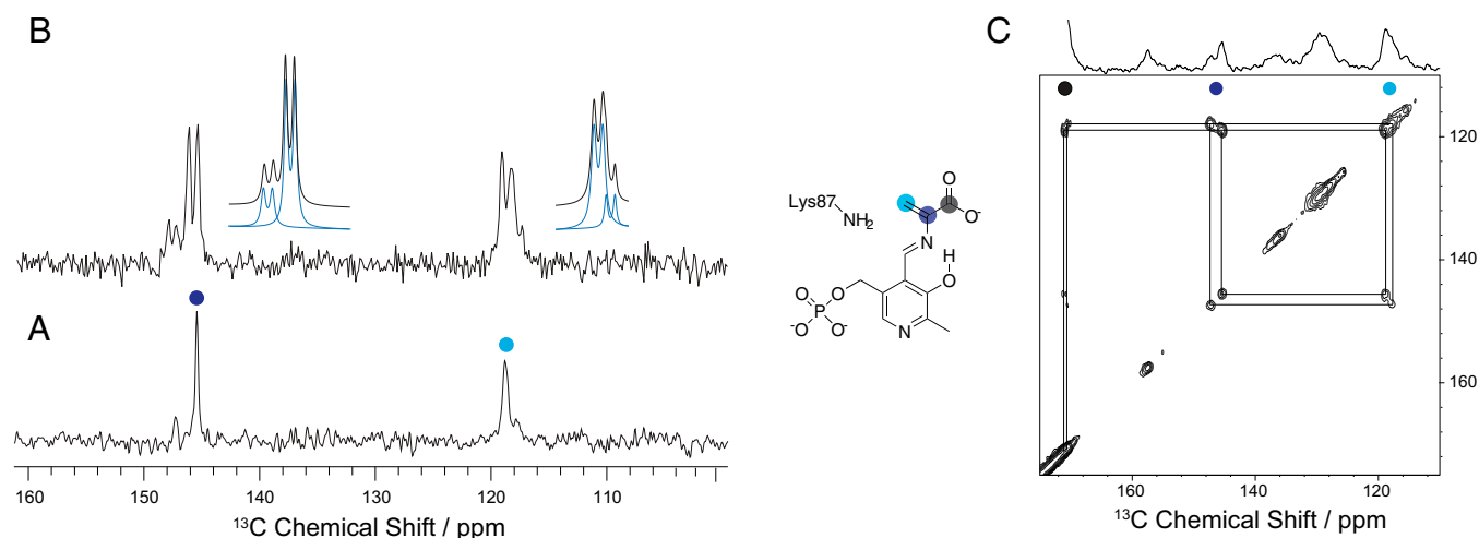
Fig. 7. ^{13}\text{C} SSNMR CPMAS spectra of microcrystalline TS E(A-A) prepared with (A) a 50:50 mixture of singly labeled 2- ^{13}\text{C} -L-Ser and 3- ^{13}\text{C} -L-Ser and (B) doubly labeled 2,3- ^{13}\text{C}_2 -L-Ser. For both, the natural abundance ^{13}\text{C} protein background has been subtracted as in Fig. 3. The \text{C}^\alpha and \text{C}^\beta resonances show a minor peak that, along with the major peak, splits into a doublet upon incorporation of doubly labeled L-Ser substrate (deconvolutions shown adjacent to the spectrum). (C) The 2D dipolar driven ^{13}\text{C} correlation spectrum of E(A-A) formed with U- ^{13}\text{C}_3 -L-Ser displays distinct cross-peaks for the major and minor resonances, indicating that they belong to two independent E(A-A) species. One-dimensional spectra acquired as in Fig. 3; 2D Spectra acquired using combined R2-driven (CORD) mixing (73) on a Bruker BioSolsids CryoProbe (74) at 14.1 T, -10^\circ\text{C} (sample temp) and 8 kHz MAS as described in Methods and Materials .
