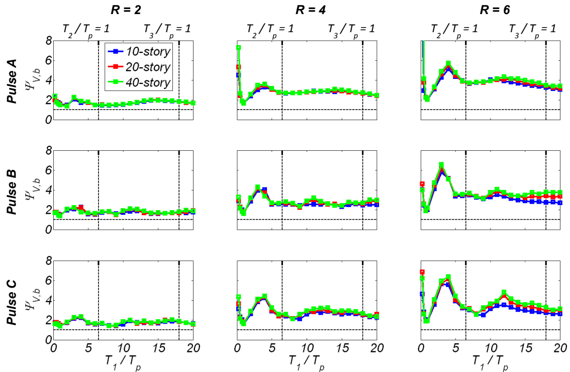
Figure 2-17. Ratio of peak base shear forces computed with NDRHA and MRSA.
