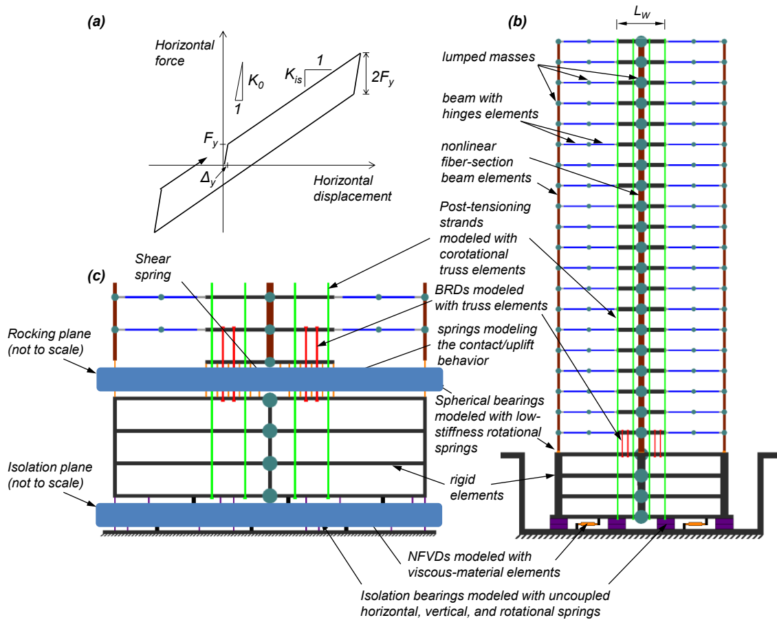
Figure 4-3. (a) Idealization of horizontal force (static) versus horizontal displacement of the two isolation systems; (b) Schematic of the numerical model of the BIRW buildings; (c) Schematic detail of isolation and rocking planes, not to scale.
