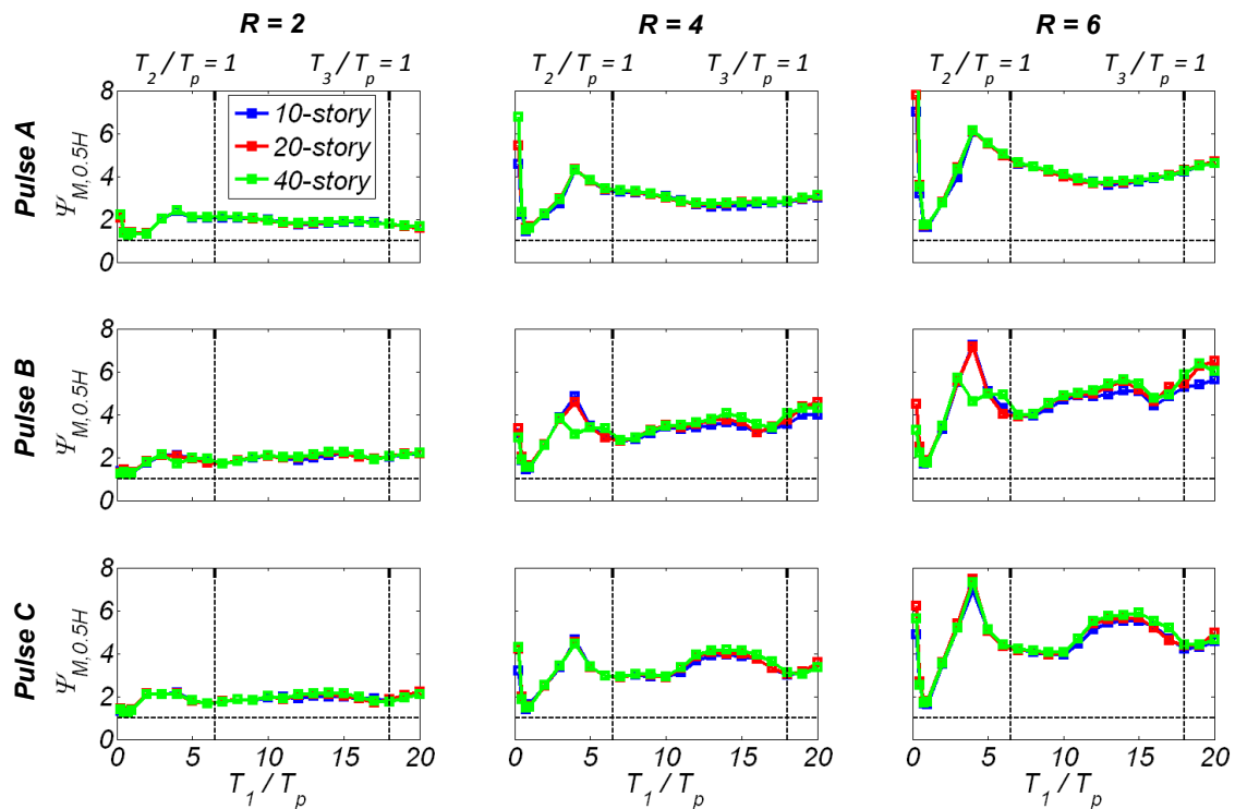
Figure 2-16. Ratio of peak mid-height bending moments computed with NDRHA and MRSA.
