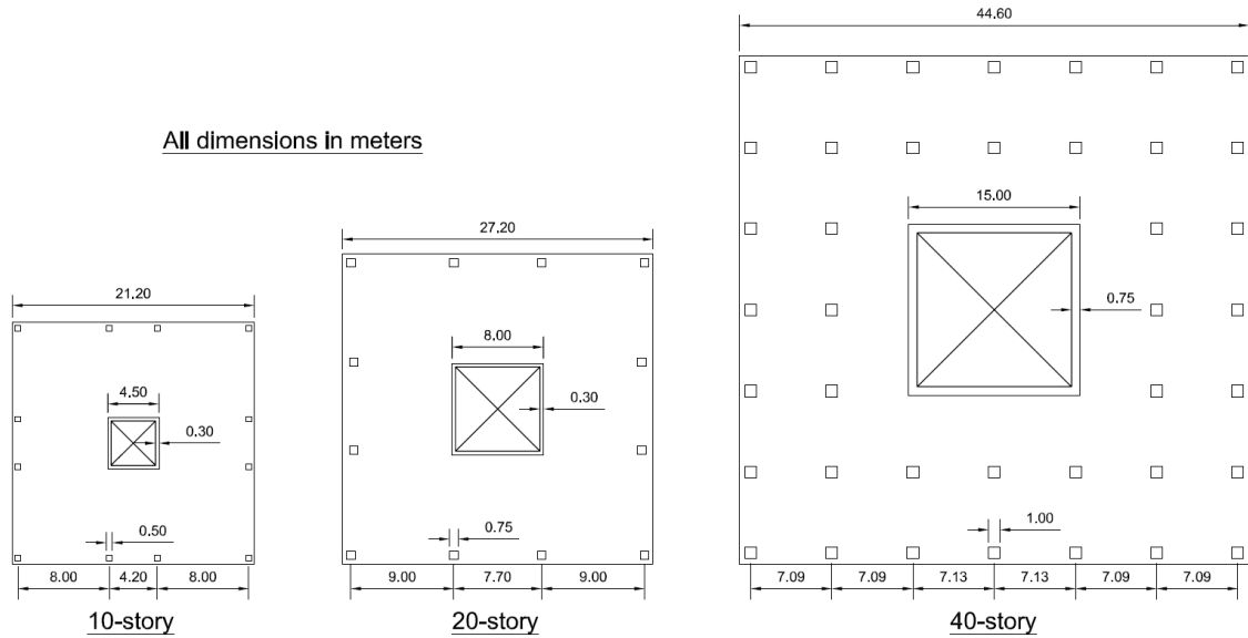
Figure 2-4. Floor plan-view of the 10-, 20-, and 40-story buildings.
