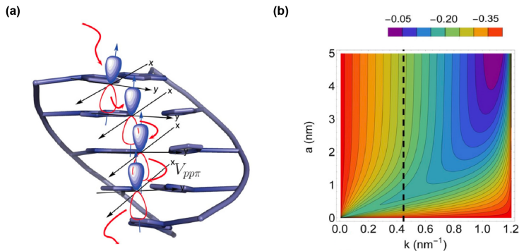
Fig. 10: Spin-orbit interaction and spin selectivity for tunneling electron transfer in DNA. (a) Schematic of DNA molecule with orbitals for electron transport. The p_z orbitals are perpendicular to the baseplanes and coupled by V_{pp\pi} Slater-Koster matrix elements. (b) Plot of spin asymmetry P_z as a function of scattering barrier length a and input momentum k . Adapted with permission from Ref. 97. Copyright 2020 by the American Physical Society.
