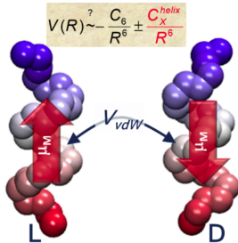
Fig. 8: In the case of chiral molecules, induction and dispersion forces encoding electric dipole-dipole interactions require additional modifications to account for exchange-mediated interactions related to the CISS effect.
