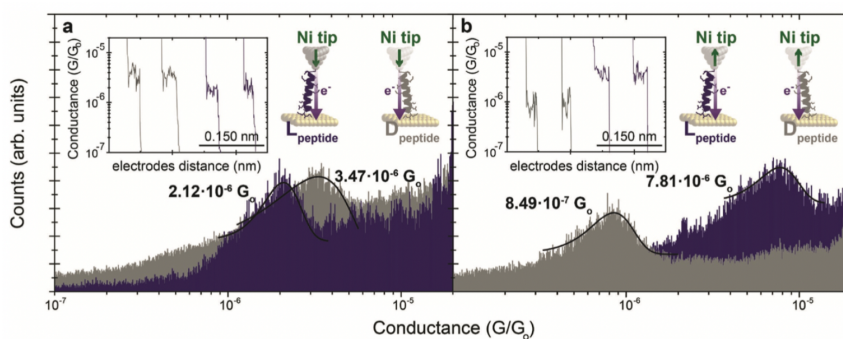
Fig. 4: Single-peptide conductance histograms from scanning tunneling microscopy break-junction measurements with Ni tips magnetized. a) down and b) up for left- versus right-handed alpha-helical peptides composed of 22 amino acid residues bridges attached to gold substrates. Insets depict representative current versus pulling traces with well-defined single-molecule plateau features. Conductance values were extracted from Gaussian fits to the histograms. Adapted with permission from Ref. 13. Copyright 2017 by John Wiley and Sons.
