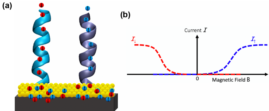
Fig. 9: (a) Functionalized gold substrates with individual peptide molecules with well defined chirality for spin selective nanodevices. (b) Application of CISS in spin rectifiers.
