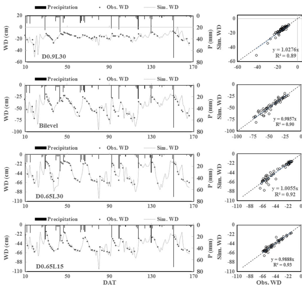
Figure 6. Temporal variations of the groundwater table depth (WD) and precipitation ( P ) during the 2015–2016 growing season (the validation period) for the four drainage systems. [Colour figure can be viewed at wileyonlinelibrary.com ]
