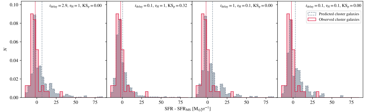
Figure A1. Example toy model-predicted cluster and observed cluster \Delta\text{SFR}_{\text{MS}} distributions for different \tau_{\text{H}} and t_{\text{delay}} timescales.
