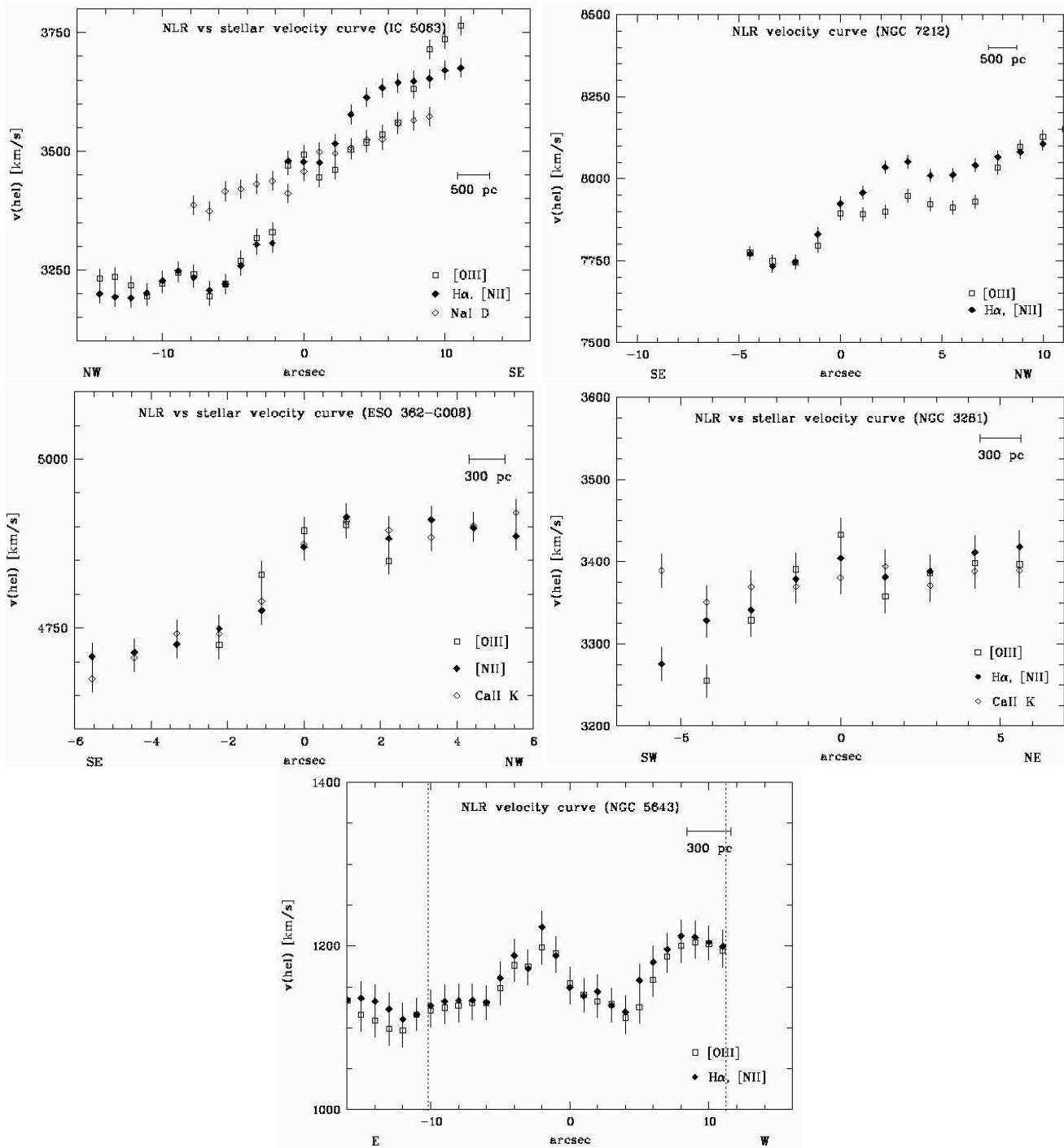
Fig. 8. Velocity fields of the Seyfert-2 galaxies IC 5063, NGC 7212, ESO 362-G008, NGC 3281, and NGC 5643. The velocities of the NLR were derived from the average value of the peak wavelengths of the H\alpha and [NII] emission lines (filled diamonds), with the exception of ESO 362-G008 where only [NII] was used. The [OIII] velocities are also shown (open squares). The stellar velocities were in most cases determined from the CaII K absorption line “peak wavelength” as seen in the “raw” spectrum (open diamonds) if visible at a good S/N with the exception of IC 5063 where NaID was used instead. For NGC 5643, the edge of the NLR as determined from the diagnostic diagrams is indicated by dotted lines.
