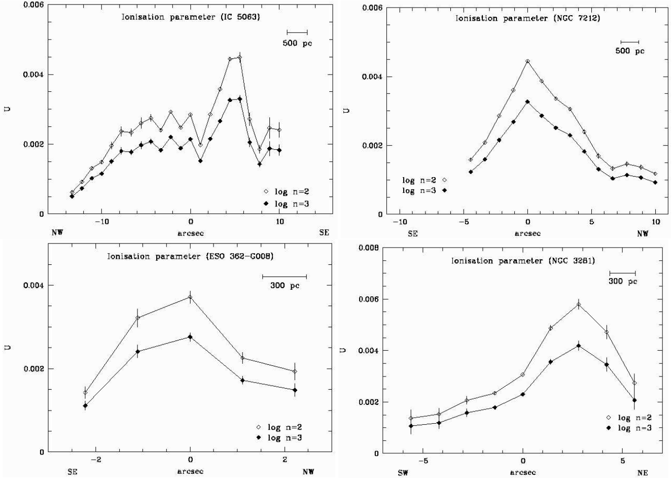
Fig. 7. Ionisation parameter derived from [O\text{II}]/[O\text{III}] ratio as a function of the distance from the nucleus for IC 5063, NGC 7212, ESO 362-G008, and NGC 3281 (open symbols: n_H = 100\text{ cm}^{-3} , filled ones: n_H = 1000\text{ cm}^{-3} ). The edge of the NLR as determined from the diagnostic diagrams is indicated by dotted lines. Note that for NGC 5643, the [O\text{I}] line was not included in the observed spectral range and we cannot present the ionisation parameter.
