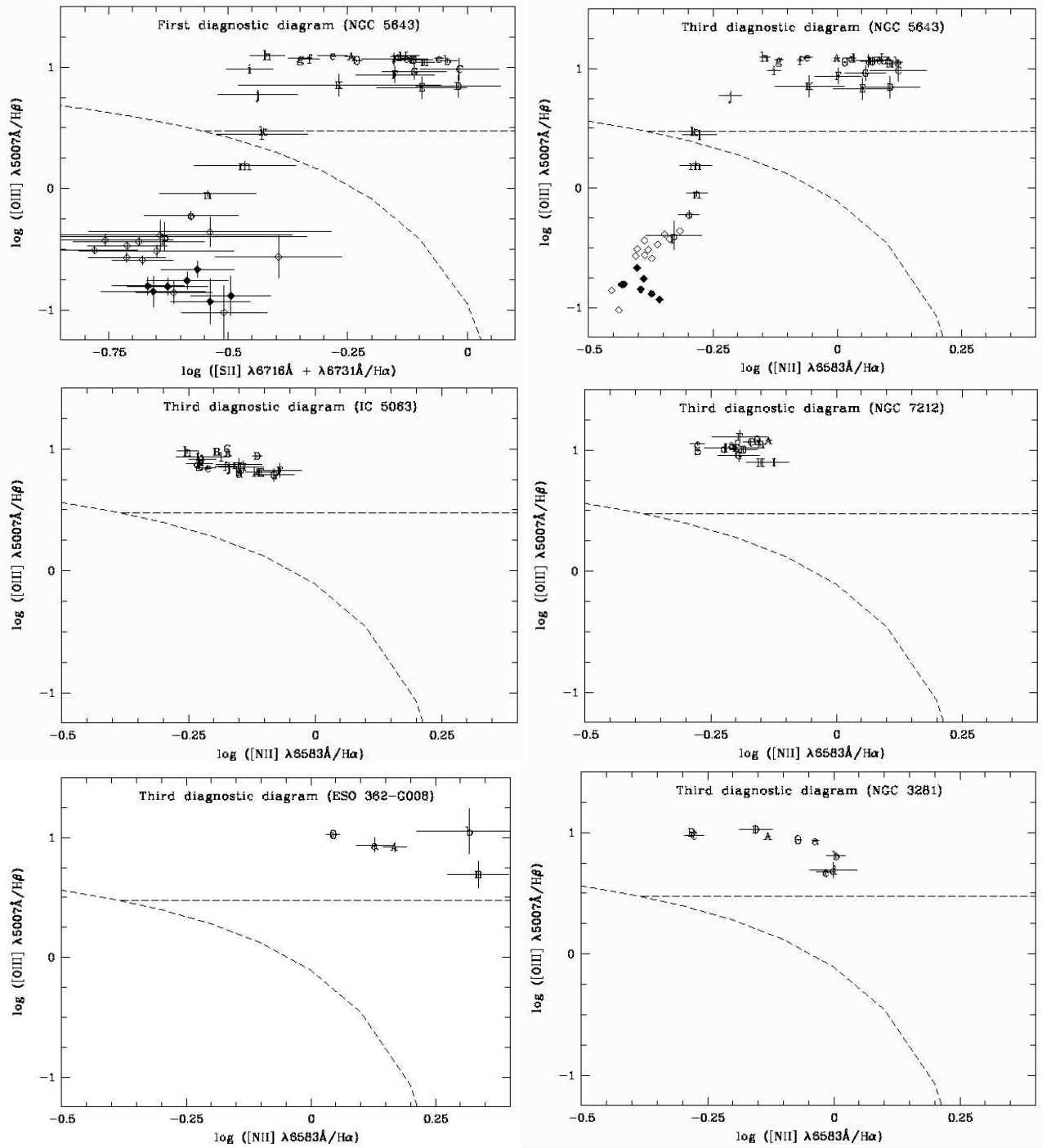
Fig. 4. Diagnostic diagrams for spatially-resolved emission-line ratios in NGC 5643 (first and third diagnostic diagram) as well as in IC 5063, NGC 7212, ESO 362-G008, and NGC 3281 (due to similarity, only third diagnostic diagram is shown).
