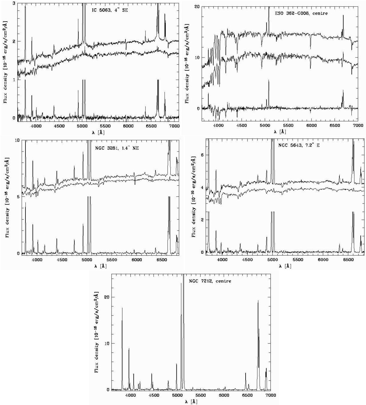
Fig. 2. Template subtraction for IC 5063, ESO 362-G008, NGC 3281, and NGC 5643. The observed (upper), the template (middle) and the template-subtracted spectra (lower spectrum) are shown. In these plots, both upper spectra are shifted vertically by an arbitrary amount. Strong emission lines are truncated in the difference spectrum. The template matches the stellar absorption lines seen in the NLR spectrum fairly well, with the exception of ESO 362-G008 for which strong Balmer absorption lines remain. For NGC 7212, no absorption features are distinguishable and thus no template was subtracted.
