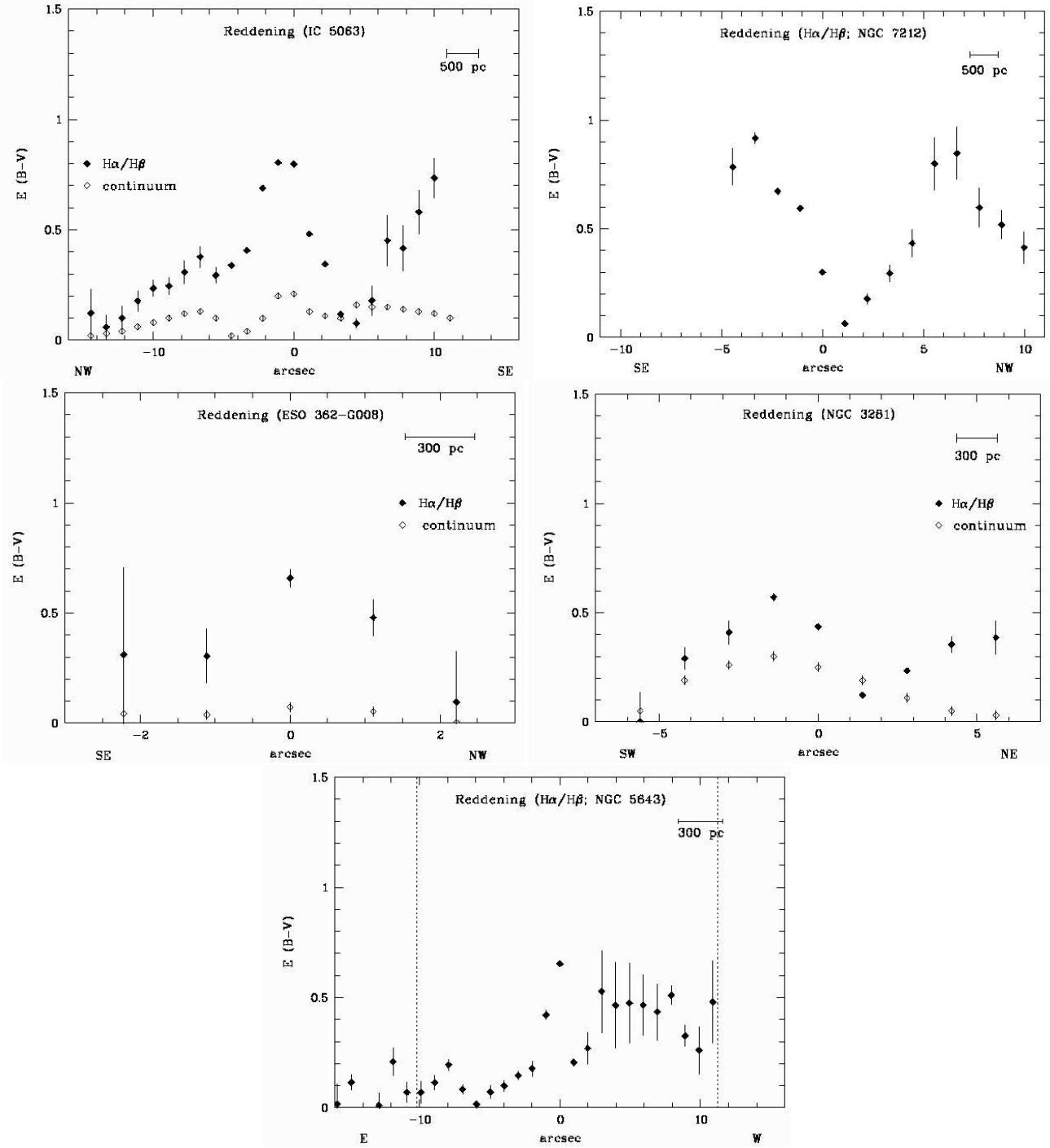
Fig. 3. Reddening distributions of the Seyfert-2 galaxies IC 5063, NGC 7212, ESO 362-G008, NGC 3281, and NGC 5643. The reddening was derived from the recombination value of the narrow H\alpha/H\beta emission-line ratio (filled symbols). For some objects, we are able to also show the reddening distribution of the continuum of the central spectra relative to the stellar template as determined during template subtraction (open symbols). For NGC 5643, the edge of the NLR as determined from the diagnostic diagrams is indicated by dotted lines.
