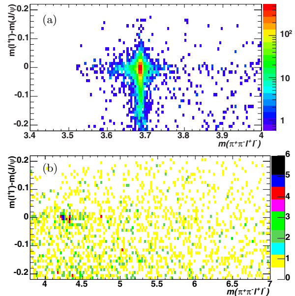
Figure 21.5.1. The scatter plot of m(\ell^+\ell^-) - m(J/\psi) vs. m(\pi^+\pi^- J/\psi) for ISR produced \pi^+\pi^- J/\psi events collected by BABAR in 123 \text{ fb}^{-1} . (a) low m(\pi^+\pi^- J/\psi) range [3.4, 4.0] \text{ GeV}/c^2 (log scale): A clean \psi(2S) signal is observed while no evidence of a X(3872) signal is seen. (b) high m(\pi^+\pi^- J/\psi) range [3.8, 7.0] \text{ GeV}/c^2 (linear scale): An enhancement around 4.3 \text{ GeV}/c^2 is found. BABAR internal, from (Aubert, 2005y) analysis.
