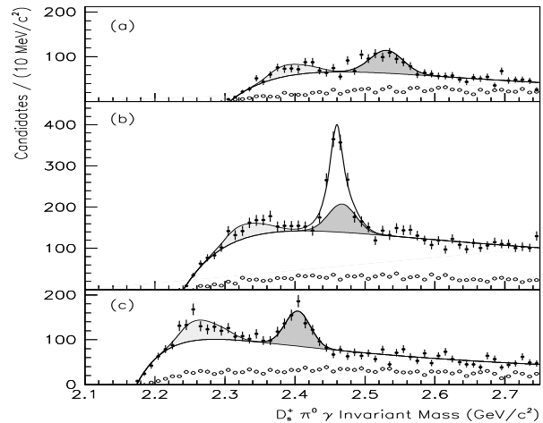
Figure 19.3.18. From (Aubert, 2006e). The M(D_s^+ \pi^0 \gamma) invariant mass distribution of candidates in the (a) upper, (b) signal, and (c) lower D_s^+ \gamma mass selection windows for (solid points) the D_s^+ signal and (open points) D_s^+ sideband samples. The curves represent the fits described in the text. The gray regions correspond to the predicted reflections from D_{s0}^*(2317)^+ (dark) and D_s^*(2112)^+ (light).
