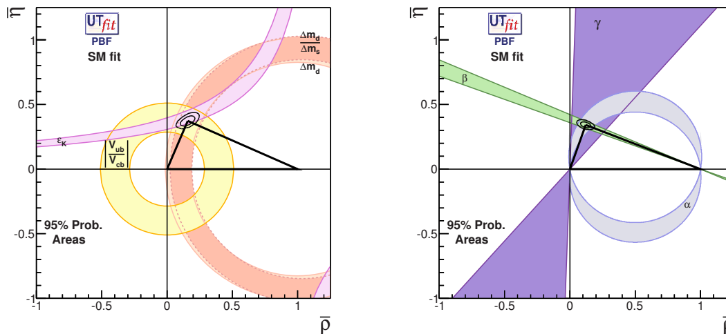
Figure 25.1.3. The consistency between the fit to CP -conserving observables and from K measurements (on the left) and the angles ( B Factory-dominated on the right) from the UTfit group. The constraints used in the left plot are the B^0 - \bar{B}^0 and B_s^0 - \bar{B}_s^0 mass differences, \Delta m_d and \Delta m_s , respectively, the measurements of |V_{ub}| and |V_{cb}| from semileptonic B decays, and the CP -violation parameter \varepsilon_K . The constraints used in the right plot are the “angles” observables, i.e. measurements of \phi_1 ( = \beta ), \phi_2 ( = \alpha ), and \phi_3 ( = \gamma ).
