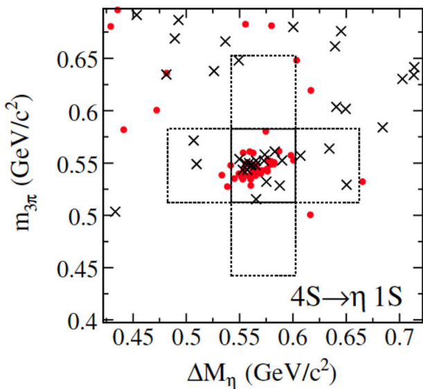
Figure 18.4.20. The distribution of M_{3\pi} vs \Delta M_{\eta} = M_{3\pi l l} - M_{ll} for \eta\Upsilon(1S) candidate events, demonstrating the observed signal (Aubert, 2008bc). Solid lines delimit the signal region, while dashed lines delimit the sideband regions used for the background estimate. Crosses represent the data from the \Upsilon(1S) \rightarrow e^+e^- sample and dots the data from the \Upsilon(1S) \rightarrow \mu^+\mu^- sample.
