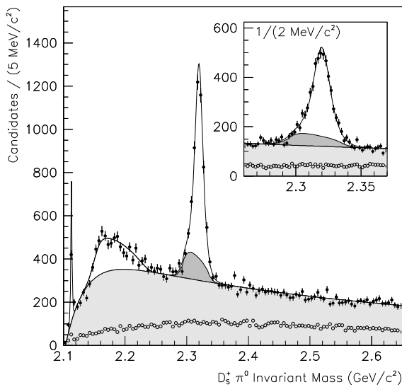
Figure 19.3.17. From (Aubert, 2006e). The invariant mass distribution for D_s^+ \pi^0 candidates (solid points) and the equivalent using the D_s^+ sidebands (open points). The curve represents the likelihood fit described in the text and includes a contribution from combinatorial background (light shade) and the reflection from D_{s1}(2460)^+ \rightarrow D_s^{*+} \pi^0 decay (dark shade). The insert highlights the details near the D_{s0}^*(2317)^+ mass. The narrow peak at threshold is due to the D_s^{*+} \rightarrow D_s^+ \pi^0 decay.
