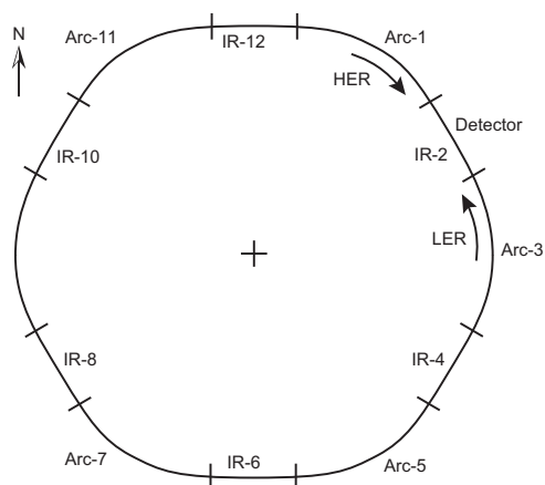
Fig. 2. Layout of the PEP-II tunnel with six straight sections (IR) and six arc sections (Arc), labeled clockwise with even numbers for the IRs and odd numbers for the Arcs. The B_{\text{ARR}} detector was located at IR-2.
