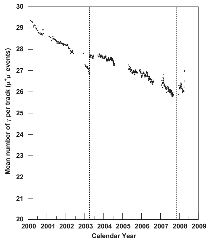
Fig. 55. DIRC: Evolution of the mean number of detected photons per track in dimuon events. The two vertical dashed lines mark the times when the PMT HV settings were raised. Note that the vertical axis is zero-suppressed: the loss over the whole data taking period is only around 10%.
