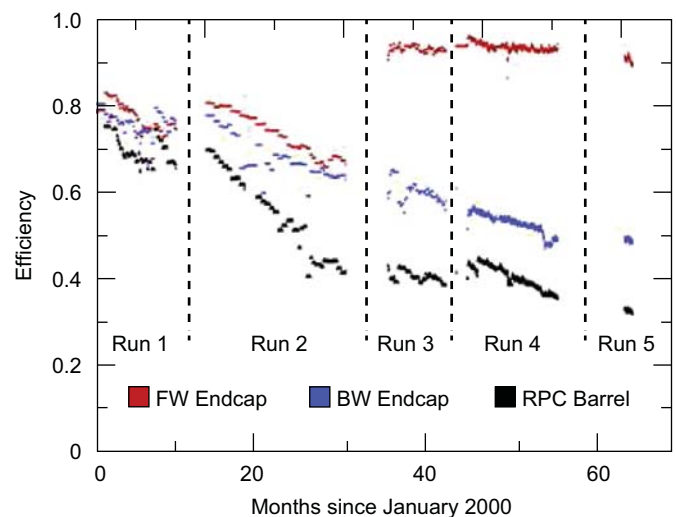
Fig. 71. Single gap RPC efficiencies determined from dimuon events accumulated during data taking as a function of time from January 2000 to May 2005. The color code differentiates data from the forward, the backward, and the barrel RPCs.
