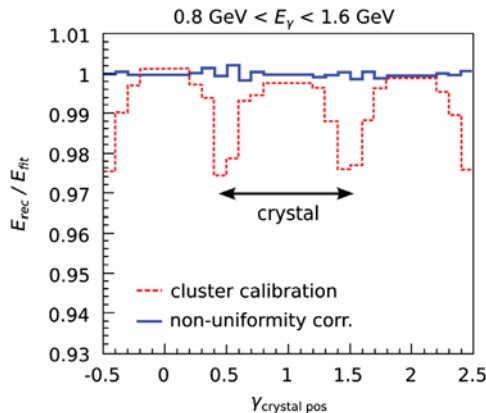
Fig. 84. Normalized response E_{\text{rec}}^\gamma/E_{\text{fit}}^\gamma across three CsI(Tl) crystals before (dashed, red) and after (solid, blue) the lateral non-uniformity correction.
