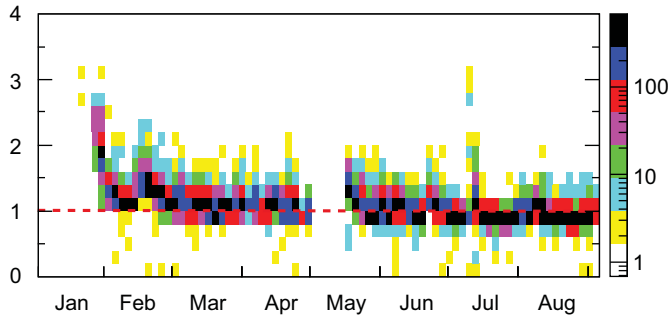
Fig. 21. DCH background monitoring: Scatterplot of the ratio of the measured total current to that predicted by PEP-II beam currents and luminosity, sampled during Run 6 (2007). The left scale shows the ratio, the right scale the color code for the number of entries per sample.
