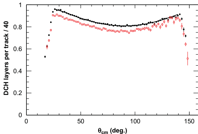
Fig. 50. DCH data from Run 6: The mean fraction of DCH layers used in the reconstruction of high-momentum tracks as a function of the polar angle \theta measured relative to the z-axis in the c.m. frame, separately for isolated muons (dots) and pions from D^0 decays (open squares).
