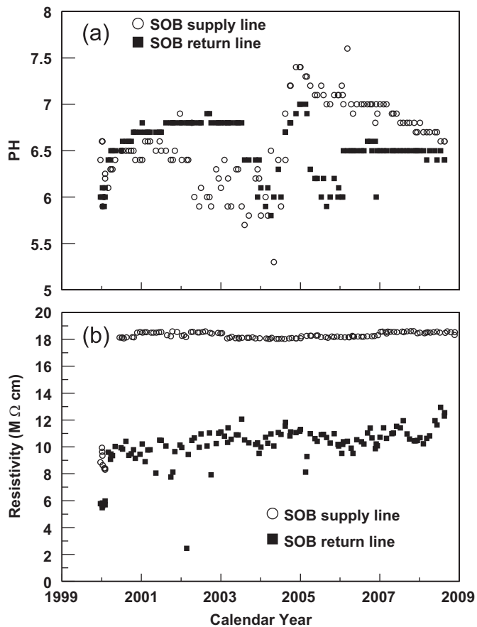
Fig. 56. DIRC water system performance over the lifetime of the experiment: (a) comparison of the pH-value and (b) resistivity of the water in the SOB supply and return lines.
