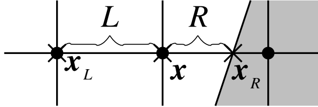
Fig. 5. Points (marked by \times ) and distances used in approximating near an internal boundary, when the shaded area is outside the domain. In this example, \varphi_L = \varphi(\mathbf{x}_L) = \varphi_{\mathbf{i}-\mathbf{e}^d}^{N,l} , and \varphi_R = \varphi(\mathbf{x}_R) is obtained from the Dirichlet boundary condition.
