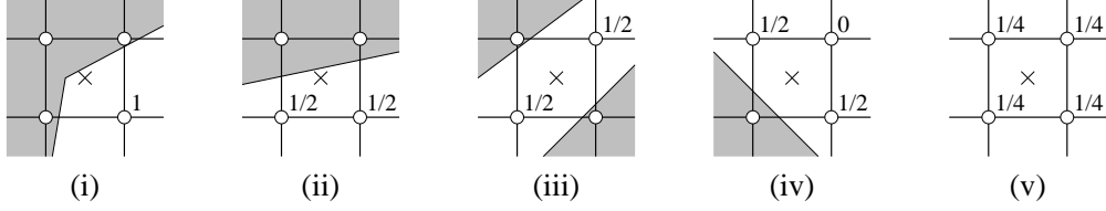
Fig. 6. The first approximation at the center node indicated by \times is a weighted average of the neighboring coarse nodes that are in the domain. Weights are indicated beside the coarse nodes.
