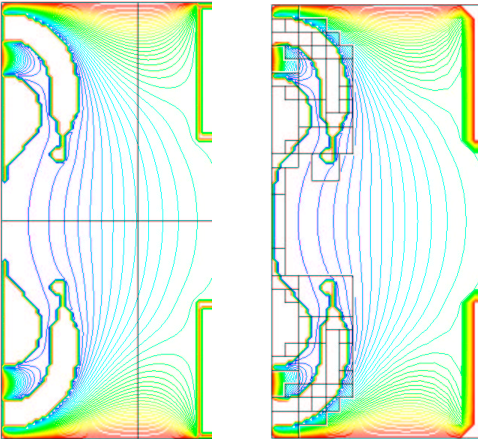
Fig. 15. Close-ups of the contour plots in Figure 14, showing the box boundaries in black, with (left) one fully refined level, and (right) two levels, with finer-level grids around emitter.
