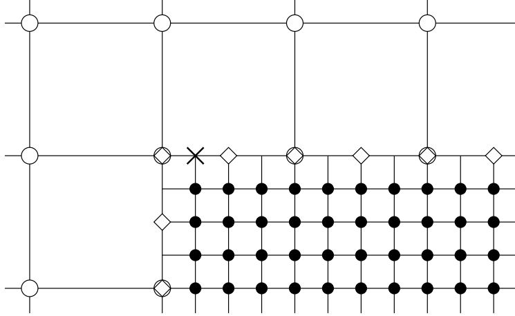
Fig. 3. A two-dimensional example with refinement ratio of 4. We interpolate to finer-level nodes on the coarse/fine interface in two stages.
