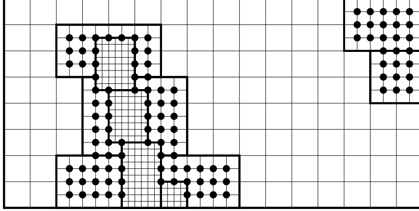
Fig. 1. A two-dimensional grid hierarchy with three levels of refinement. The valid nodes at the middle level are indicated by \bullet .
