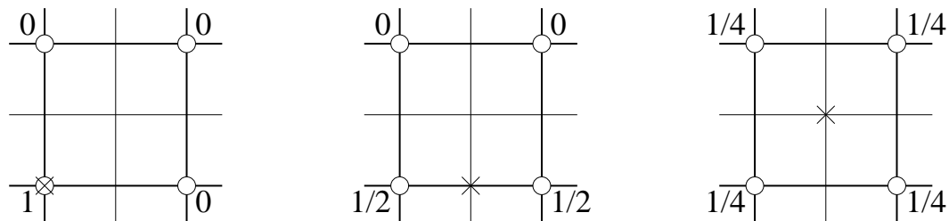
Fig. A.4. Interpolation in two dimensions to a fine node indicated by \times , when the refinement ratio is 2. Weights are shown on the coarse nodes in three cases.
