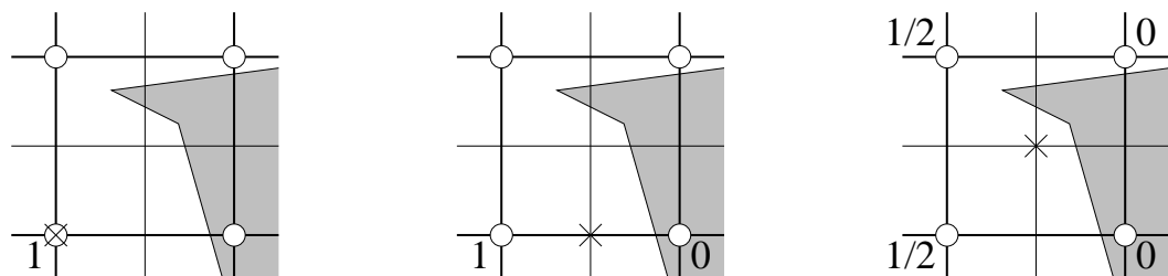
Fig. A.5. Interpolation in two dimensions to a fine node indicated by \times , when the refinement ratio is 2. The shaded area is outside the domain. For three different fine nodes, weights are shown on the coarse nodes used for interpolation. Compare with Figure A.4.
