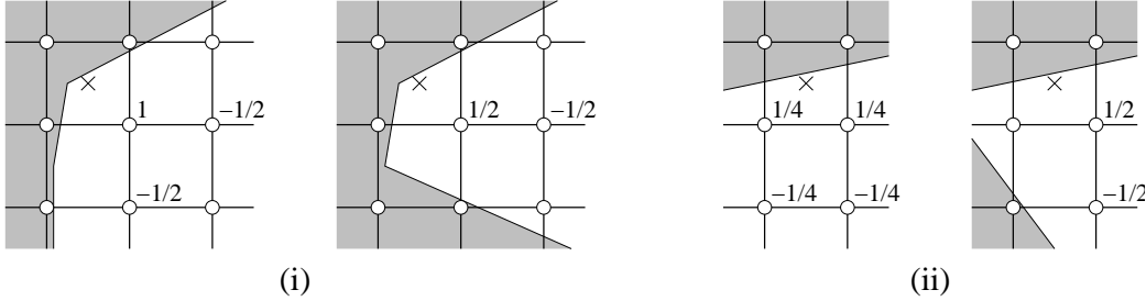
Fig. 7. One-sided bilinear correction to approximation at center node \times . Weights of the correction are indicated beside the coarse nodes.
