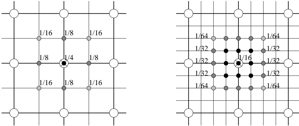
Fig. A.1. Averaging down to the center coarse node indicated by \times , in two dimensions. Weights are indicated at the fine nodes, with different shadings for different weights.
