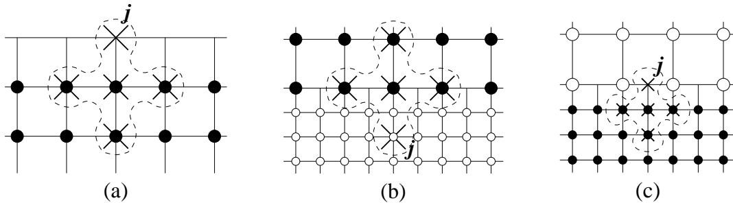
Fig. 2. Cases in which data at non-valid nodes is needed in computing the discrete Laplacian at a valid node. Nodes of the stencil are indicated by \times , valid nodes at the current level by \bullet .
