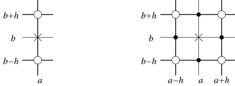
Fig. 4. Interpolating a value at the point (a, b) , marked \times , from coarse nodes indicated by \circ .
