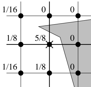
Fig. A.2. Weights of fine nodes in averaging to the coarse node indicated by \times . The shaded area is outside the domain. Some nodes have weight 0, even though they are in the domain, because there is no path to them from \times following edges that lie entirely in the domain, without backtracking.
