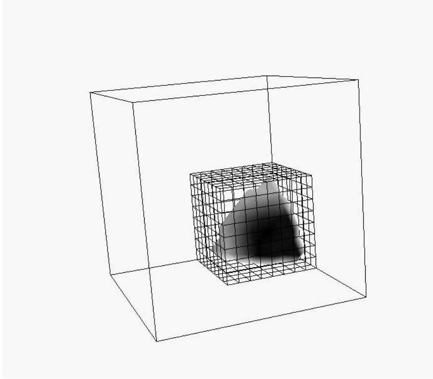
Fig. 11. In our examples, we solve for the field outside the shaded region due to a point charge within it. We solve on nested hierarchies of grids in the configuration shown with two levels of refinement.
