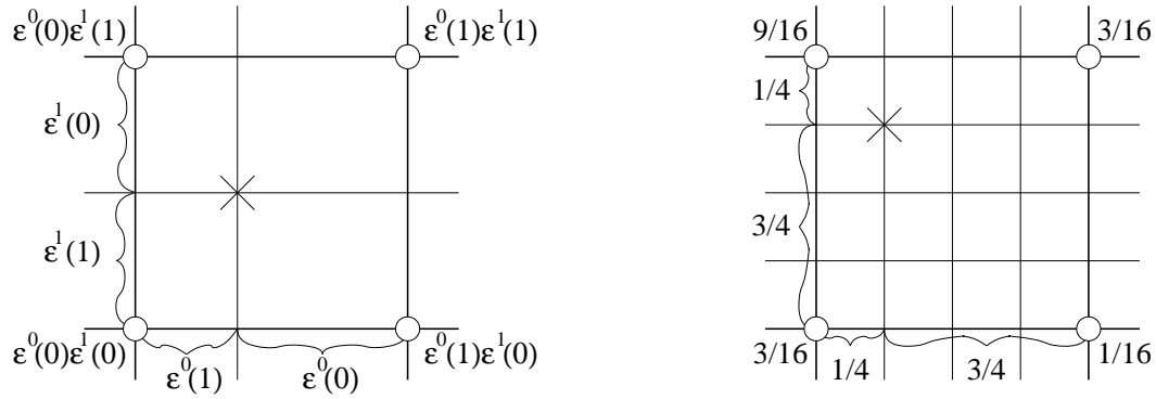
Fig. A.3. Left: Length fractions and weights of coarse nodes in bilinear interpolation in two dimensions to the fine node indicated by \times . Right: An example with refinement ratio of 4.
