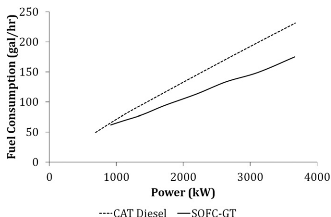
Fig. 10. Comparison of SOFC-GT and diesel engine fuel consumption across operating range.
