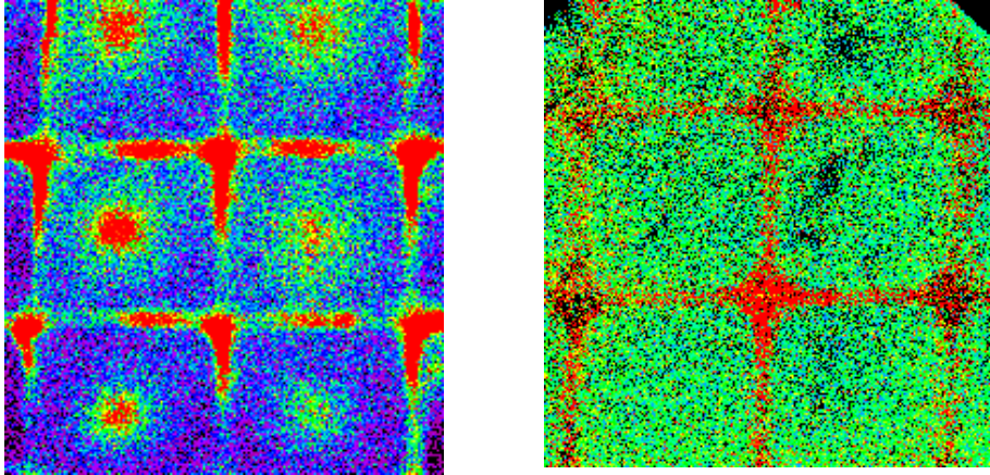
Figure 4 High explosive matrix with a 18 μm nickel grid pressed onto the front surface. Left side is without, right side with charge compensation.
