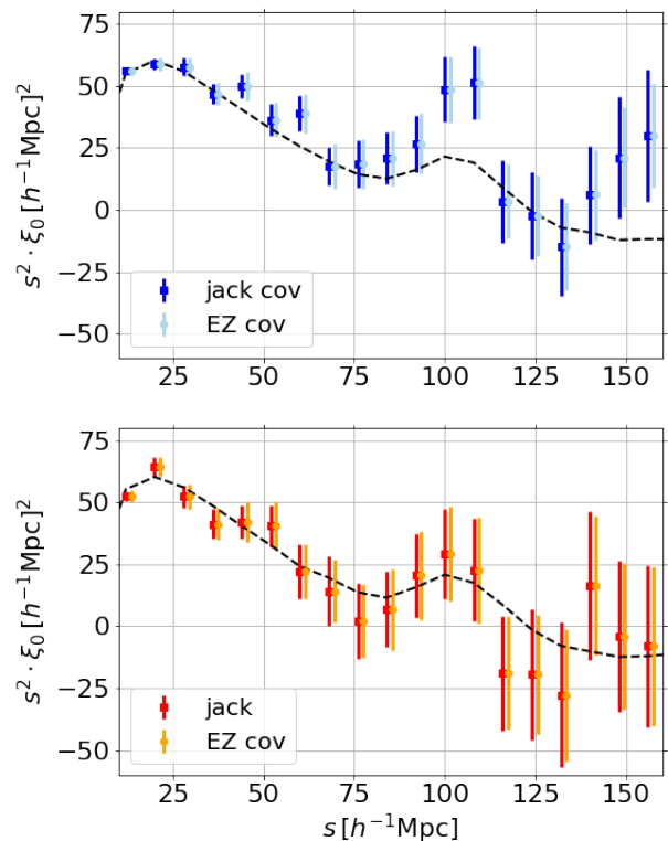
Figure 11. Monopole of the auto-correlation of eBOSS DR16 quasars in the NGC (top) and SGC (bottom) with error bars coming from the 100 jackknife realisations and from the 1000 EZ mocks.
