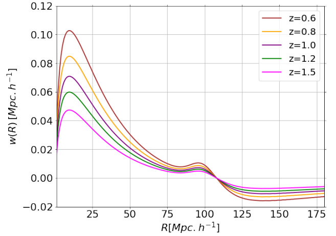
Figure 1. Evolution with redshift of the template for the matter projected correlation function following equation 9 and with a bin width of 1 h^{-1} \text{Mpc} .
