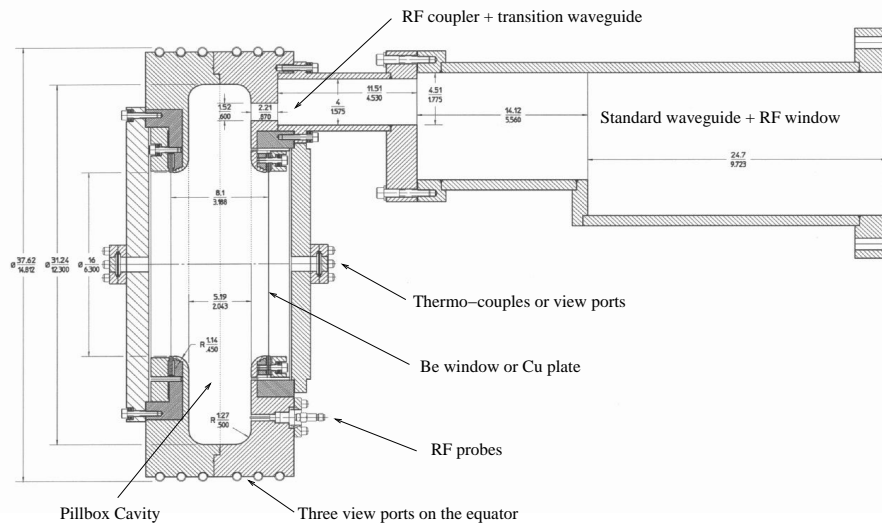
Figure 1. Cross section of the 805 MHz high power test cavity.
