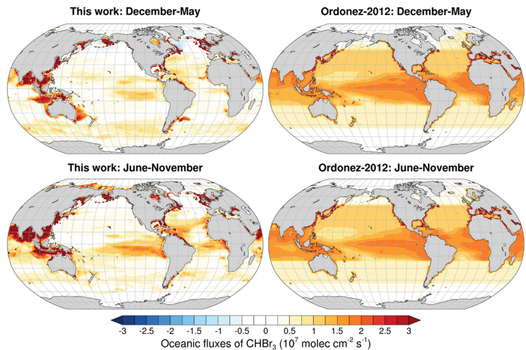
Figure 8. December–May and June–November averages of the oceanic emission fluxes of CHBr 3 predicted in this work (left) compared to a top-down inventory from Ordóñez et al. (2012; right). Warmer colors indicate upward fluxes (i.e., the ocean is net emitting), while colder colors indicate downward fluxes (i.e., the ocean is net sink).
