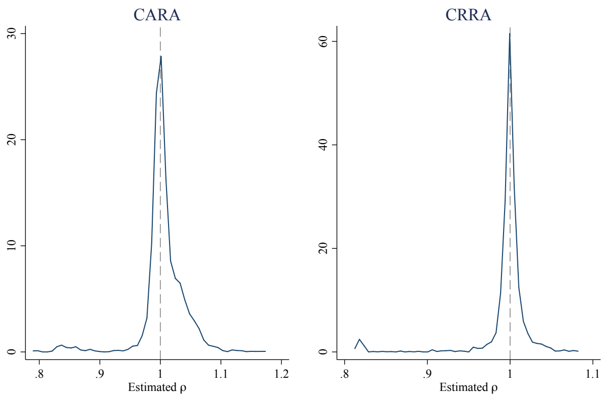
Figure 3: Normalized time preference parameter \rho
