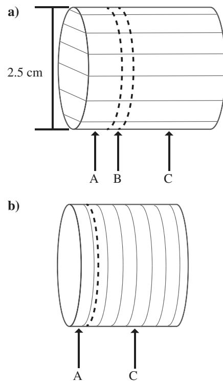
Figure 2. A schematic representation of the subsampling of the (a) horizontal and (b) vertical plugs. The labeled subsamples are: (A) excess material used for geochemical analysis, (B) a 0.2 cm thick coin for XRD experiments, and (C) an approximately 2.0 cm long plug for acoustic experiments.
