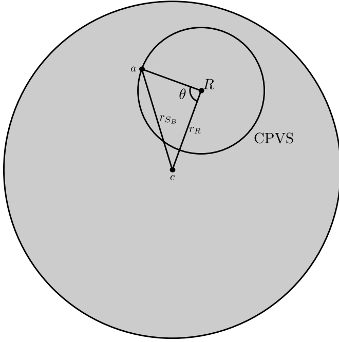
Figure 20. Calculation of location of CPVS, labeled r_{SB} , with respect to the center of the SN. The quantity r_R is the magnitude of the vector cR and r_{SB} is that of ac .
