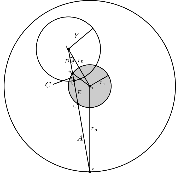
Figure 22. Case I geometry. The value of A corresponds to the magnitude of the vector xw , E to wv , C to vu , D to ut , r_c to ou , and r_s to xo . Only E and C contribute to the intensity of the ray since A and D lie outside the emitting core.
