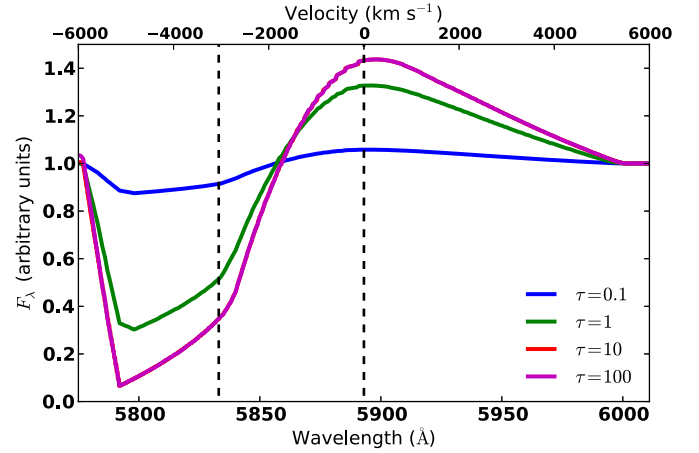
Figure 8. Flux profiles for Na I D in SYNOW, with photospheric velocity 3000 \text{ km s}^{-1} and spatially constant optical depth. The maximum velocity of the line-forming region is 6000 \text{ km s}^{-1} . The right dashed vertical line indicates the rest wavelength of the Na I D line ( \lambda 5892 ), and the left vertical line indicates the blueshifted rest wavelength of Na I D at the photospheric velocity. The \tau = 10 and \tau = 100 profiles overlap almost exactly and are indistinguishable in this figure. Unlike the profiles in Figure 7, the emission peak in the SYNOW case remains fixed at the line rest wavelength regardless of the optical depth. (A color version of this figure is available in the online journal.)
