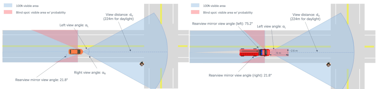
Figure 1. Visible areas and blind spots when driving without intelligent vehicle technology, passenger cars (left) and trucks (right)
