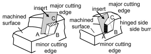
Fig. 32. Tool exit order sequence affects the burr formation condition [56].
