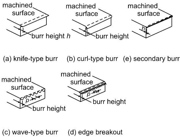
Fig. 11. Five types of burrs observed in face milling [29].
