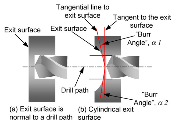
Fig. 18. Burr formation when drilling intersecting holes according to Min [105].
