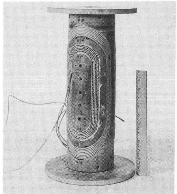
Figure 5. Dipole No. 8 and 8A prior to adding outer helium channels and flux-return yoke.
