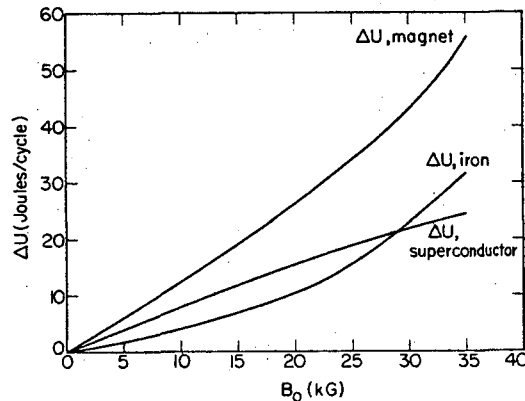
Figure 3. Energy loss measurements, Dipole No. 8.
