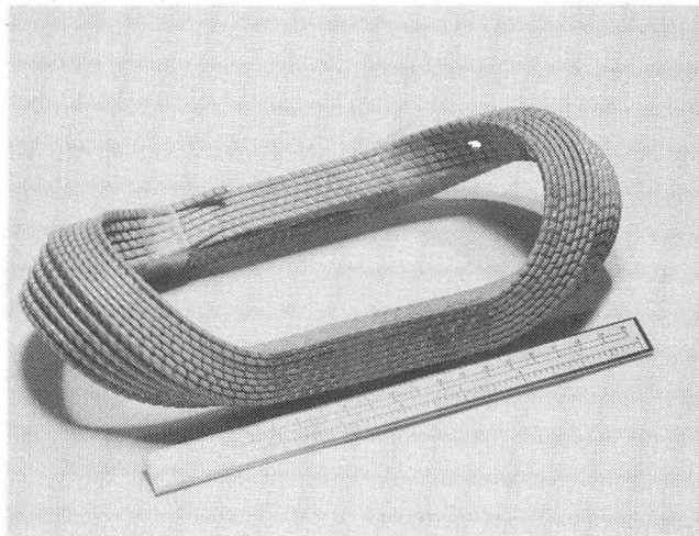
Figure 7. Experimental coil for Dipole No. 9 made by a new method.
