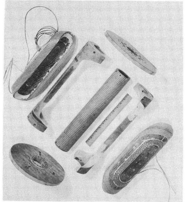
Figure 4. Parts for Dipole No. 8 and 8A.
