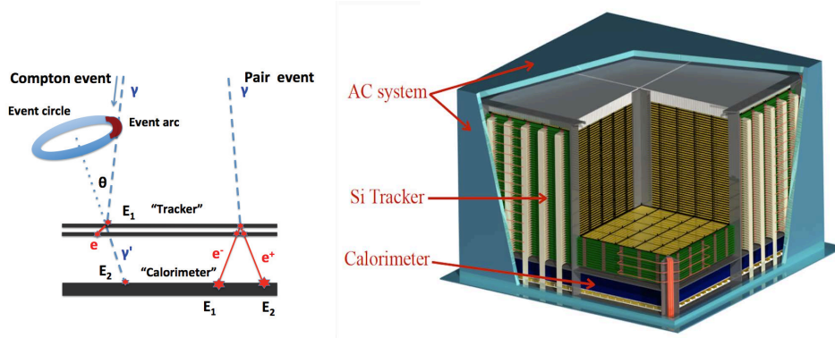
Figure 1.2.2: Left: Representative topologies for a Compton event and for a pair event. Photon tracks are shown in pale blue, dashed, and electron and/or positron tracks are in red, solid. Right: Overview of the e-ASTROGAM payload.
