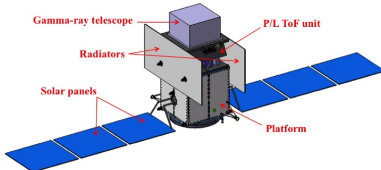
Figure 1.2.1: e-ASTROGAM spacecraft with solar panels deployed.
