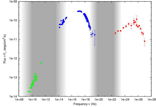
Figure 2.13.2: SED of Mrk 421 measured in multi-wavelength campaigns including Fermi and MAGIC telescopes [243]. The green circles corresponds to the radio emission from an extended region of the jet. The blue and red circles denote synchrotron and SSC emission respectively. The shaded area corresponds to the most appropriate frequency band, in order to constrain \gamma_{\min} .
