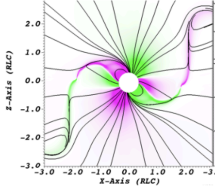
Figure 6.4.1: Current J \cdot B in a near-force-free magnetosphere. The pink/green color indicates current along/opposite the local magnetic field direction. Current flows out of the polar regions and in from the current sheet. From [663].
