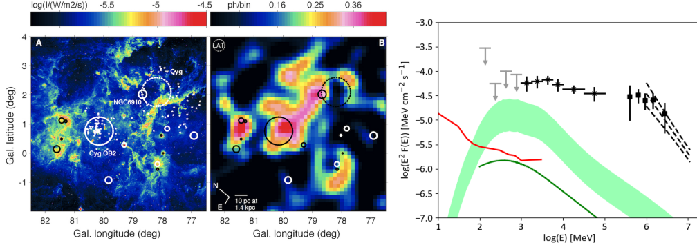
Figure 3.3.1: Left: 8 \mu\text{m} intensity map of the Cygnus X region from MSX showing the heated contours of the superbubble. OB stars (white stars), OB associations (white circles), and the supernova remnant \gamma Cygni (dashed circle) are overlaid [307]. Center: Fermi -LAT photon count map of the same region in the 10-100 GeV band. The 50-pc-wide excess coincident with the bubble signals a cocoon of freshly accelerated CRs [307]. Right: Energy spectrum of the Cygnus cocoon emission as detected by Fermi -LAT (crosses), ARGO-YBG (squares), and MILAGRO (dashed lines). The curves show model expectations from normal Galactic CRs spreading the ionized gas (green band) or up-scattering the stellar and interstellar light fields (green curve). The sensitivity of e-ASTROGAM (red curve) is given for one year of effective exposure in the Galactic disc. Adapted from [306, 307].
