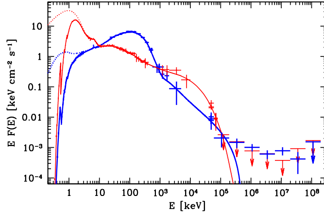
Figure 6.7.1: Broad-band X-ray/gamma-ray spectra for Cyg X-1 in the hard (blue heavy symbols) and soft (red thin symbols) states. The data at < 10 MeV (attenuated by X-ray absorption) are from BeppoSAX and CGRO, while the data at \geq 40 MeV are from Fermi/LAT. Data are compared to hybrid-Comptonization accretion-flow models [696]. The observed emission above \sim 100 MeV in the hard state is dominated by the jet. The dotted curves at soft X-rays show the unabsorbed models.
