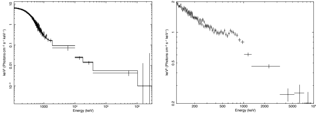
Figure 6.7.2: Left: Simulated 10^{-5} -s e-ASTROGAM average hard-state spectrum of Cyg X-1 assuming contributions from thermal Comptonization in the accretion flow at low energies and from synchrotron emission in a jet at high energies, as in Fig. 6.7.1. Right: Simulated 10^{-5} -s spectrum of an X-ray binary with a power law of \Gamma = 2.5 and a broad line from annihilation of e^{\pm} [716] at the temperature of kT \simeq 100 keV.
