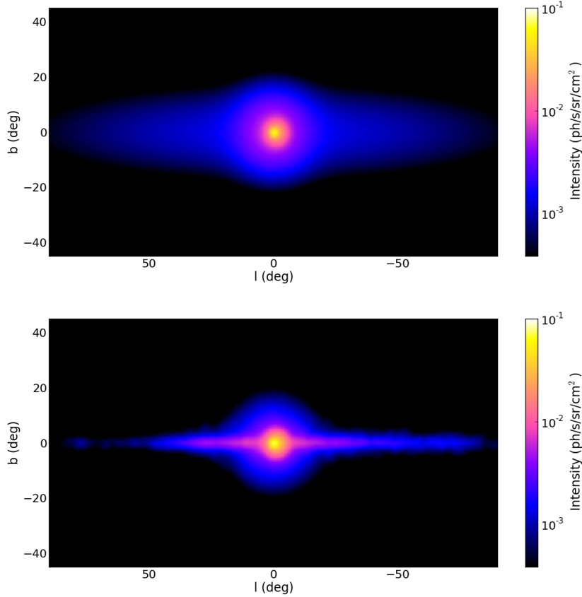
Figure 5.5.1: Simulated e-ASTROGAM observations of the 511 keV emission, obtained for an exposure of 1 year of the inner Galactic region, assuming (top) the model proposed by [600] with a thick disk and (bottom) a model with the disk of [613] and the point source and bulge components of [614].
