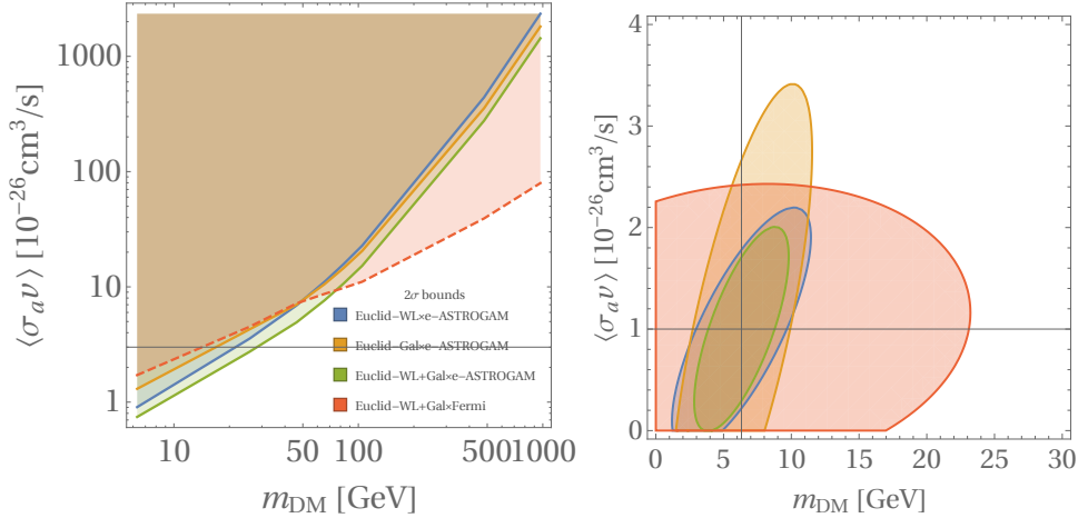
Figure 4.10.1: Left panel: Expected 2\sigma bounds on the DM annihilation cross section, \langle\sigma_a v\rangle , versus its mass for a DM candidate annihilating into bottom quarks. The blue line is derived for the cross-correlation of e-ASTROGAM with Euclid weak-lensing cosmic shear, the yellow instead considers the Euclid galaxy clustering, and green line is their combination. The dashed red line shows the bound expected with Euclid data (weak lensing together with galaxy clustering) combined with Fermi-LAT 10 year data dating Right panel : Expected 1\sigma joint marginal error contours on WIMP parameters for e-ASTROGAM gamma-ray data cross-correlated with Euclid (same colour code as in left panel). We chose a WIMP candidate with fiducial DM mass of \sim 6 GeV and \langle\sigma_a v\rangle = 10^{-26} \text{ cm}^3/\text{s} .
