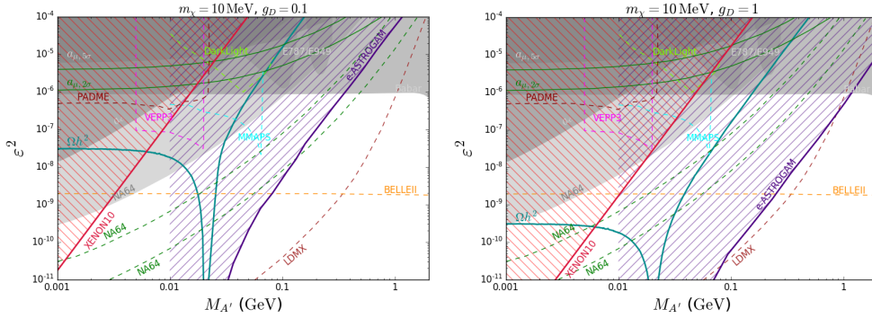
Figure 4.2.2: MeV DM complementarity : Bounds on the plane \epsilon^2 versus dark photon mass. Direct detection and e-ASTROGAM exclusion regions are shown in red and purple hatched regions respectively. The correct relic density curve with turquoise lines for DM mass m_\chi = 10 MeV and two different values for the dark coupling g_D , g_D = 0.1 (left panel) and g_D = 1 (right panel). Existing (projected) bounds resulted from dark photon searches are displayed with gray regions (dashed lines).
