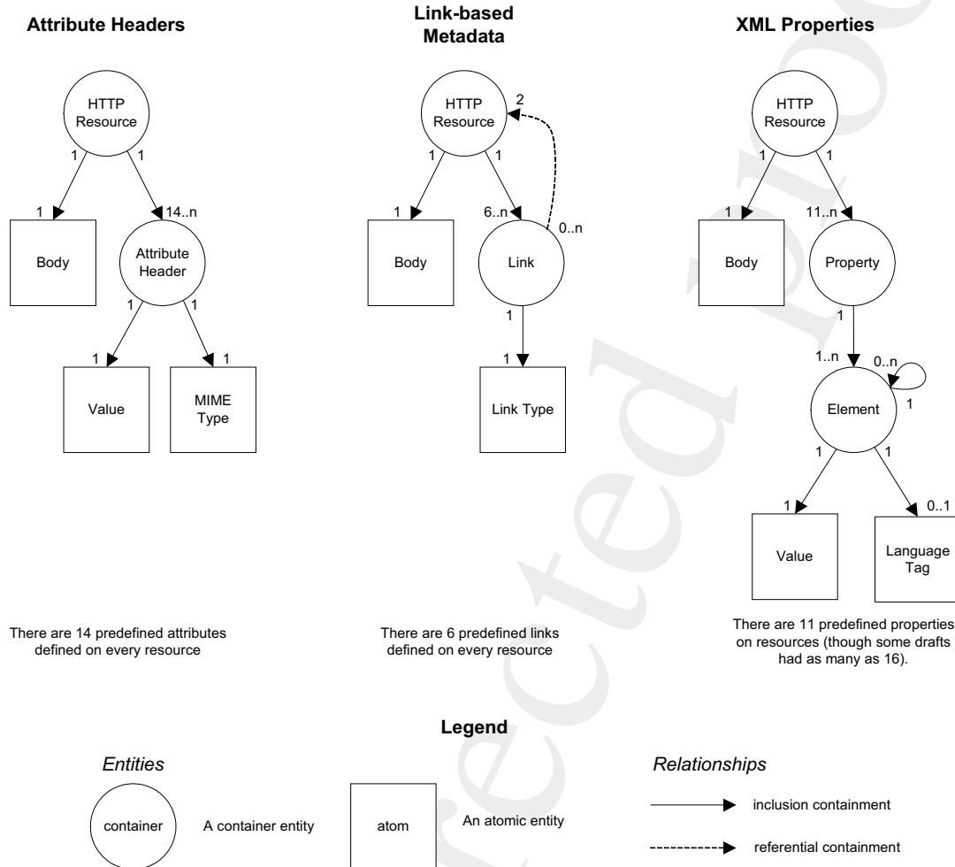
Figure 2. Containment models of WebDAV metadata designs.
