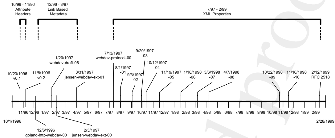
Figure 1. Timeline showing the publication date of individual WebDAV protocol drafts (bottom), and the timespans for successive metadata designs (top). Consistent naming and version numbering of WebDAV specifications did not begin until draft-ietf-webdav-protocol-00, released in July 1997. While all of these drafts are now expired IETF Internet Drafts, and hence no longer available from the IETF, archived copies can be accessed via the WebDAV Working Group [41].
