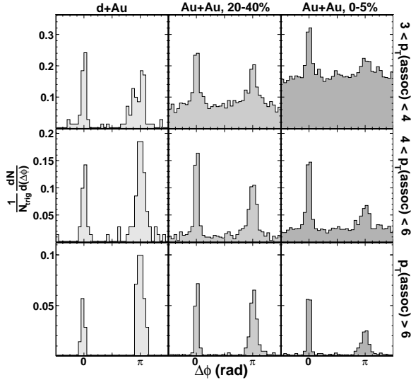
Figure 8. Azimuthal correlations between a trigger particle with p_T > 8 GeV/c and an associated particle in different p_T ranges (in GeV/c) for dAu and mid-peripheral and central AuAu collisions [28].
