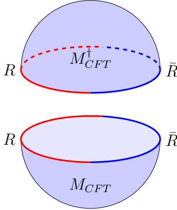
Figure 1. The manifold M_{CFT} (bottom) that we use in the Euclidean path integral to prepare our holographic state |\psi\rangle and the CPT-conjugate manifold M_{CFT}^\dagger (top). Sewing the two together along their boundaries defines the manifold M_{double} := M_{CFT}^\dagger M_{CFT} . If the state is time-symmetric, then M_{CFT}^\dagger is equivalent to M_{CFT} , the two manifolds are exchanged by the relevant notion of time-reversal, and this symmetry leaves invariant the boundary \partial M_{CFT} = \partial M_{CFT}^\dagger of M_{CFT} , \partial M_{CFT}^\dagger . The surface \partial M_{CFT} is partitioned into regions R (red) and \bar{R} (blue).
