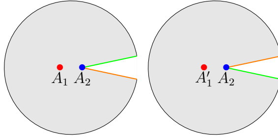
Figure 4. Using the same projection as for the n = 1 figure at left in figure 3, we show two pieces of a corresponding saddle that for A_1 \neq A'_1 describes an off-diagonal contribution to the second Rényi entropy S_2 . The full saddle is constructed by sewing the two pieces together along edges of the same color; i.e., we may first identify the two green edges and then identify the two orange edges. Note that this particular saddle contains only one copy of the surface \gamma_2 and so cannot be ‘off-diagonal’ in A_2 .
