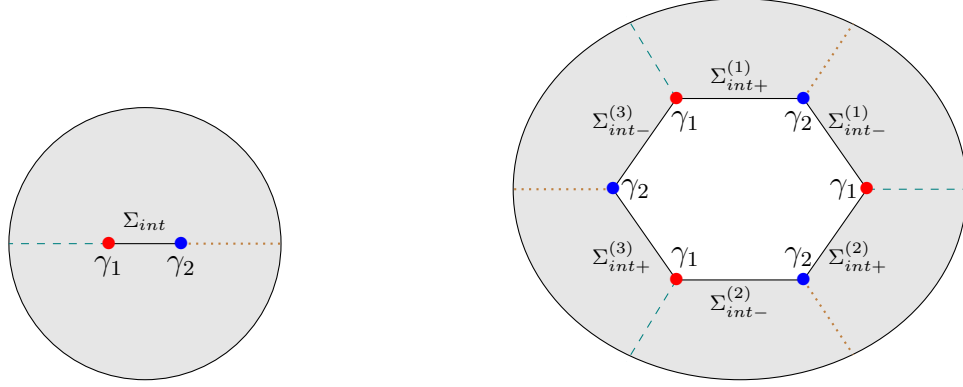
Figure 3. Left: A two-dimensional projection of an n = 1 solution with two extremal surfaces \gamma_1, \gamma_2 (having areas A_1 and A_2 ) and a surface \Sigma_{int} stretching between them. Right: An n -fold cover of the figure at left for the case n = 3 after cutting open a slit along \Sigma_{int} . The 2n copies of \Sigma_{int} are labeled \Sigma_{int\pm}^{(i)} , where i = 1, \dots, n . Saddles for the Rényi entropy are formed by identifying \Sigma_{int+}^{(i)} with \Sigma_{int-}^{(\pi(i))} for some permutation \pi . After making such identifications, the number N_2 = n - n_2 of copies of \gamma_2 that remain is the number C(\pi) of cycles generated by \pi , while the corresponding N_1 = n - n_1 is C(\tau \circ \pi) where \tau is the counterclockwise cyclic permutation. The asymmetry is due to the numbering of replicas, which breaks the natural symmetry between the dashed lines (separating replicas) and dotted lines (separating the two halves of each replica).
