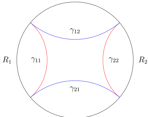
Figure 5. Two competing extremal surfaces when R = R_1 \cup R_2 is a pair of intervals on the boundary of the AdS_3 vacuum. The homotopic RT surface \gamma_d = \gamma_{11} \cup \gamma_{22} and the non-homotopic RT surface \gamma_o = \gamma_{12} \cup \gamma_{21} are shown respectively in red and blue. The case shown sits precisely at the RT phase transition, where \gamma_d and \gamma_o are related by a \pi/2 rotation.
