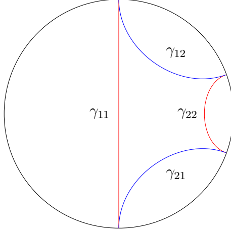
Figure 6. The same geodesics as in figure 5 after applying an \text{AdS}_3 isometry to move the boundary-anchors \gamma_{11} to the poles \theta = 0, \pi . This configuration allows us to compute changes in length by applying results from section 4.
