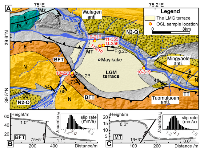
Figure 2. (a) Simplified geologic map of the Mayikake basin (location in Figure 1c): BFT-Biertuokuoyi Frontal Thrust, MT-Mayikake Thrust, and TT-Tuomuluoan Thrust. The prefix “LED” of OSL sample number is omitted. Same legend as Figure 1. (b and c) Topographic survey profiles across thrust scarps and Monte Carlo simulation results of the BFT and MT, respectively.
