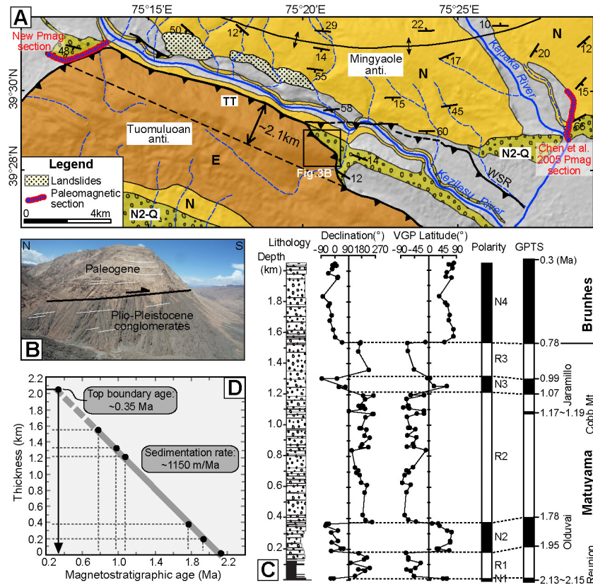
Figure 3. (a) Geologic map of the Tuomuluoan Thrust (TT) and surrounding area showing a minimum overthrusting width of \sim 2.1 km between Paleogene and Pleistocene strata. WSR-1985 Wuqia earthquake surface rupture. Location map in Figure 1c. Same legend as Figure 1. (b) Field photo of the TT outcrop, exposing Paleogene units overthrusting Pleistocene conglomerate. Outcrop location marked in Figure 3a. (c) Magnetostratigraphy of the Pleistocene conglomerate section as correlated with the time scale of Lourens et al. [2004]. (d) Thickness as a function of magnetostratigraphic age. Upward extrapolation of the nearly uniform sedimentation rate seen from \sim 2.15 to 0.8 Ma implies an age of \sim 0.35 Ma for the top of the section.
