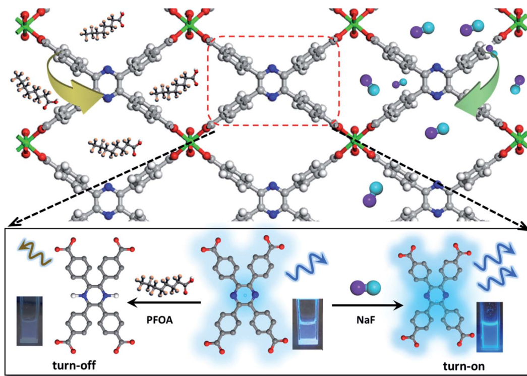
Scheme 1 The structure of \text{In}(\text{tcpcp}) (top) and schematic presentation of its luminescence switchable turn-off response toward PFOA (bottom left) and turn-on response toward F^- ions (bottom right). Color codes: C grey; N blue; F light blue; O red; In green; Na purple; and H white.
