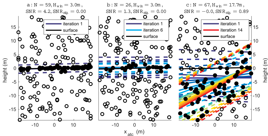
Fig. 4. ATL06 photon selection refinement process. Photon selection refinement process shown for three cases based on simulated ATL03 photons (open circles: all photons; filled circles: final ATL06-selected photons): a) segment where the signal has moderate-strength, where ATL03-flagged photons (not shown) defined a narrow surface window; b) segment with a weaker signal, where six iterations were required to converge on the surface; c) segment with no ATL03-flagged photons, where, after 14 iterations, the algorithm converged to a wide, sloping window centered 5 m below the surface. In all plots, solid colored lines show the segment height for different iterations, proceeding in spectrum order from blue to red. Dashed lines show the bounds of the surface window, with colors matching the surface-fit color. (For interpretation of the references to color in this figure legend, the reader is referred to the web version of this article.)
