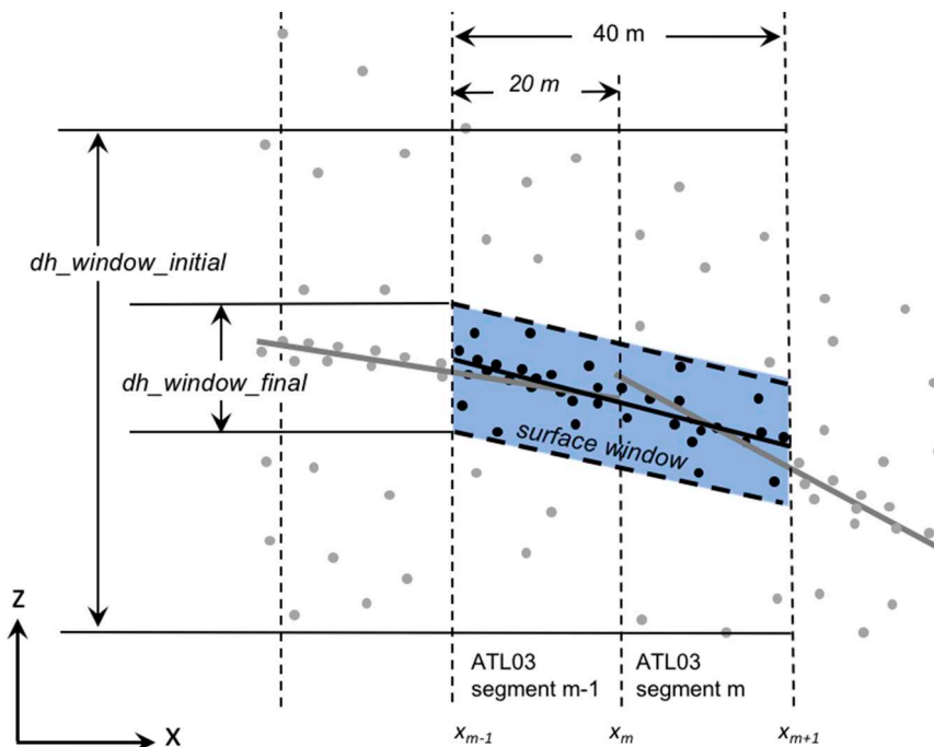
Fig. 3. ATL06 segment fitting: Along-track segments fit to photon heights (gray circles) as a function of along-track distance ( x ) for segment m (black line) and neighboring segments m + 1 and m - 1 (gray lines). Photons selected by the ATL06 photon-refinement algorithm for reference point m are shown in black.
