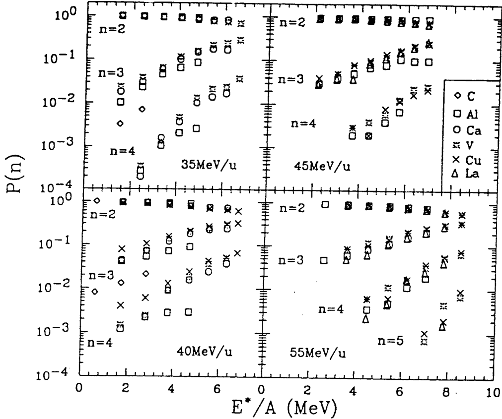
Fig. 4: Proportion of 2-3-4-5 fold events as a function of the excitation energy per nucleon for the systems studied at 4 different energies.
