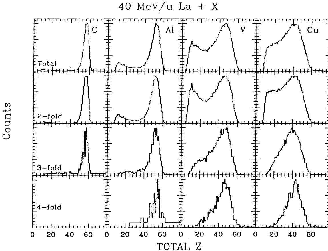
Fig. 2: Total detected charge for some of the systems measured at 40 MeV/u as a function of the multiplicity in the exit channel.
