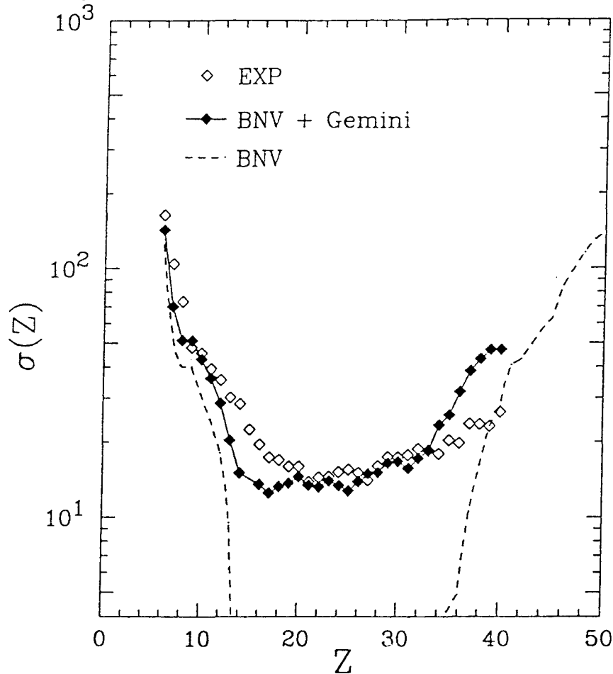
Fig.5: Comparison of the experimental and calculated charge distribution for the system La + Al at 55 MeV/u. No normalization factor has been applied to the simulation. The statistical errors on experimental data are smaller than the diamonds and the errors related to the extraction procedure are smaller than 20% except above Z = 35 where the cross section can be underestimated by up to 60% due to the reduced angular coverage for the very heavy fragments.
