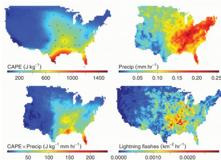
Fig. 1. Mean maps of CAPE, precipitation, CAPE times precipitation, and lightning flashes. For the year 2011, maps are shown of mean (top left) CAPE from the SPARC radiosonde data, (top right) precipitation from the National Weather Service River Forecast Center data, (bottom left) product of the top two maps, and (bottom right) CG lightning from the NLDN data. For CAPE, means are calculated by averaging all 00 and 12 GMT soundings; circles denote the locations of radiosonde releases. For precipitation and lightning, means are calculated by averaging over 22-02 and 10-14 GMT.
