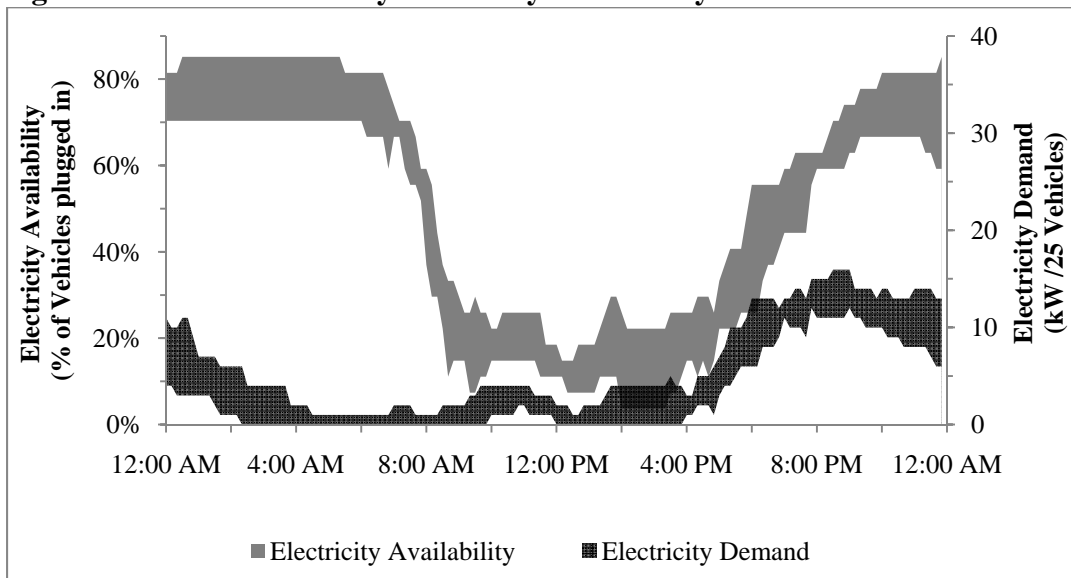
Figure 9 Observed Weekday Electricity Availability and Demand
