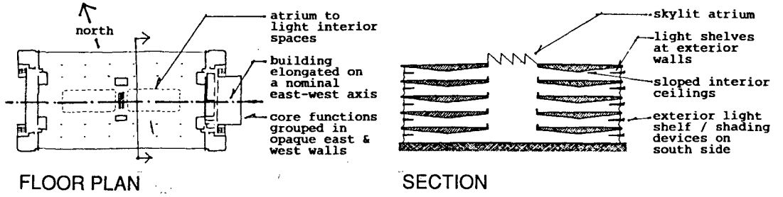
Figure 1. Building Plan and Section
