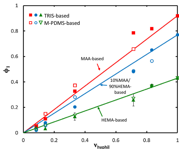
Fig. 1. Equilibrium water volume fraction, \phi_1 , as a function of the solvent-free volume fraction of hydrophilic monomer, v_{hyphil} , for HEMA-(triangles), MAA-(squares), and 10% MAA/90% HEMA-based (circles) SiHys. Filled and open symbols denote TRIS- or M-PDMS-based SiHys, respectively. Typical error bars are shown. Lines are drawn according to theory.
