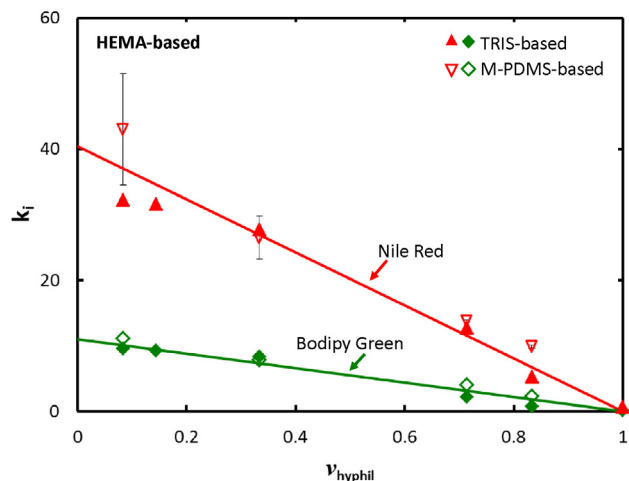
Fig. 4. Oleophilic-solute partition coefficients, k_i , as a function of the solvent-free volume fraction of hydrophilic monomer, v_{hyphil} , for Nile Red (triangles) and Bodipy Green (diamonds) in HEMA-based SiHys. Filled and open symbols denote TRIS- or M-PDMS-based SiHys, respectively. Typical error bars for Nile Red are shown. Error bars for Bodipy Green are the size of the data points. Lines are drawn according to theory.
