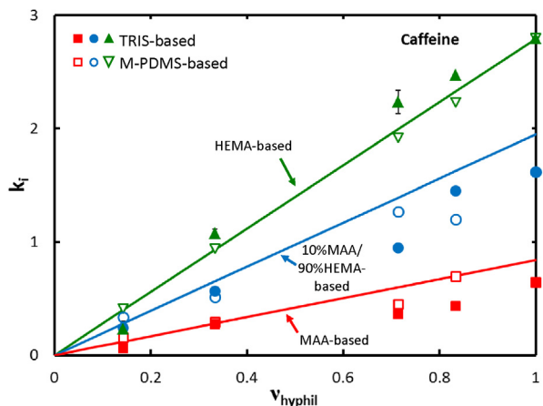
Fig. 3. Caffeine partition coefficients, k_i , as a function of the solvent-free volume fraction of hydrophilic monomer, v_{hyphil} , for HEMA-(triangles), MAA-(squares), and 10% MAA/90% HEMA-based (circles) SiHys. Filled and open symbols denote TRIS- or M-PDMS-based SiHys, respectively. Typical error bars are shown. Lines are drawn a priori according to theory.
