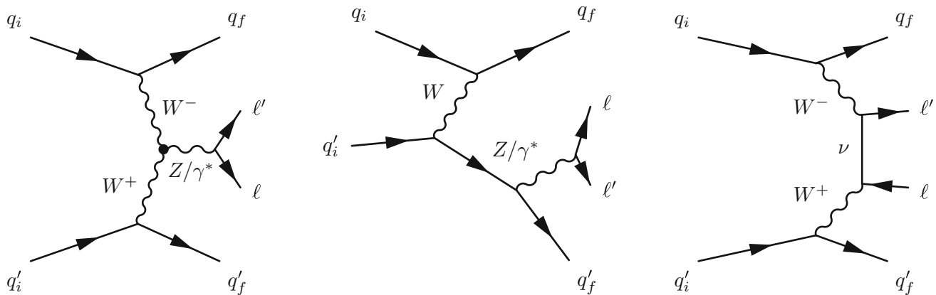
Fig. 1 Representative Feynman diagrams for dilepton production in association with two jets from purely electroweak contributions: (left) vector boson fusion, (middle) bremsstrahlung-like, and (right) multiperipheral production
