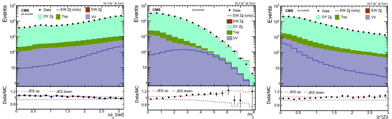
Fig. 4 Distribution for (left) the difference in the azimuthal angle and (middle) difference in the pseudorapidity of the tagging jets for ee events, with R_{p_T}^{\text{hard}} \geq 0.14 . The z^* distribution (right) is shown for
