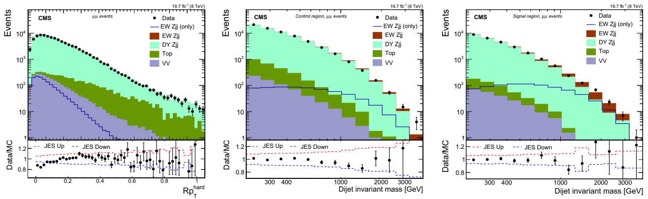
Fig. 3 Distribution for (left) R_{p_T}^{\text{hard}} and M_{jj} for \mu\mu events with (middle) R_{p_T}^{\text{hard}} \geq 0.14 (control region) and (right) R_{p_T}^{\text{hard}} < 0.14 (signal region). The contributions from the different background sources and the signal are shown stacked, with data points superimposed. The panels
