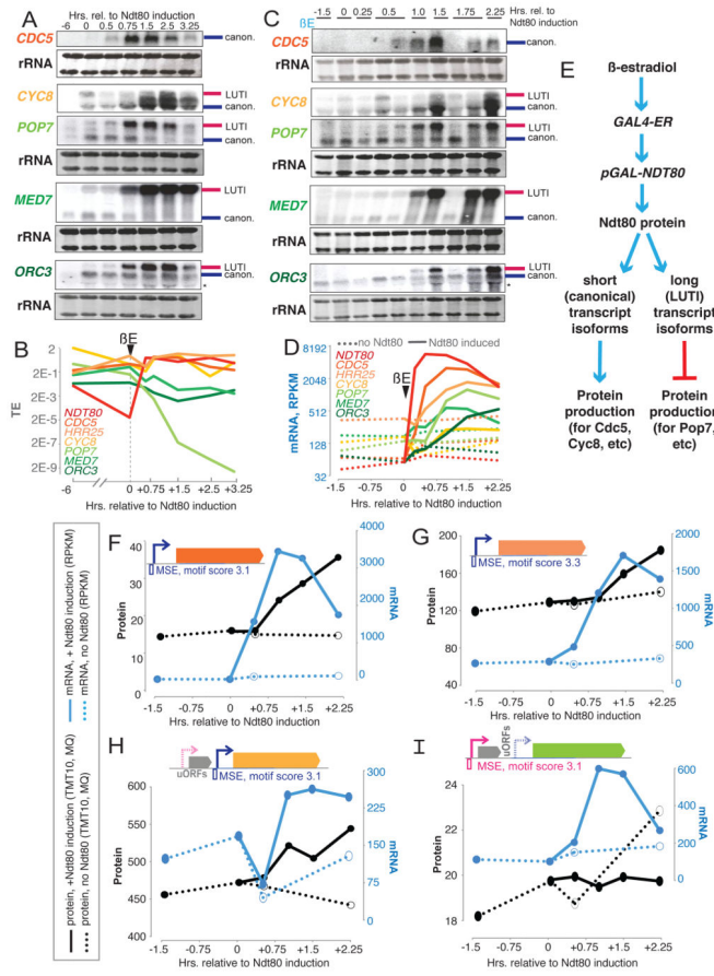
Figure 5. A single transcription factor coordinately induces long, translationally silent transcript isoforms and canonical transcripts, with opposing effects on protein production. A) Northern blotting reveals rapid increases in mRNA following Ndt80 induction for canonical Ndt80 target, CDC5 , the canonical transcript isoform of CYC8 , and long isoforms of POP7 , MED7 , and ORC3 . Pink and blue bars at the right of blots indicate canonical and LUT1 isoforms. B) These increases in mRNA result in decreased TE for POP7 , MED7 , and ORC3 , while CDC5 and the short CYC8 isoform are better translated after Ndt80 induction. C) Northern blotting reveals Ndt80-dependence to induction of CDC5 , the canonical transcript isoform of CYC8 , and long isoforms of POP7 , MED7 , and ORC3 , *denotes a background band. D) mRNA abundance increases for traditional and long, poorly translated Ndt80 transcript isoform targets occur with similar timing and are dependent on Ndt80. Dotted lines show mRNA abundances without addition of \beta -estradiol. Solid lines show measurements with. E) Outline of experiments in A) and C) and expected effects on gene expression. F–I) mRNA (blue) and protein (black) are shown with (solid line) and without (dotted line) Ndt80 induction for F) canonical targets CDC5 and G) HRR25 , H) the canonical transcript isoform of CYC8 , and I) POP7 LUT1 . Note that induction of canonical mRNAs results in an Ndt80-dependent increase in mRNA and protein, while induction of the POP7 LUT1 results in an Ndt80-dependent increase in mRNA but decrease in protein, relative to no Ndt80 induction. See also Fig. S5, Table S4, Table S5.
