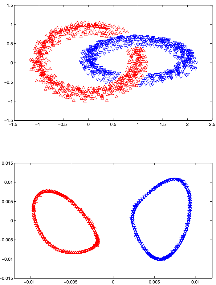
Figure 2: Data objects form two interlocking rings (but not touching each other) in 3D Euclidean space (top). In SPCA space (bottom), the rings separate. Objects self-aggregate into much thinner rings.
