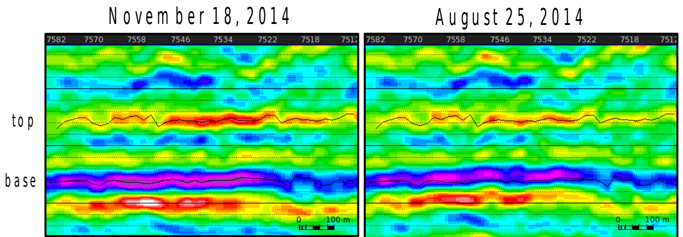
Figure 7. Two east-west cross-sections through the time-lapse seismic monitoring data. As in Figure 6, the numbers at the top of the plot are track numbers, with each track spaced 10 meters apart. Coherent time shifts and amplitude changes are visible for reflections at and below the base of the reservoir. The top and base of the reservoir correspond to the pink and blue lines in Figure 6. The red values and purple values are the minimum and maximum values that lie in the range 1-2 ms. Reprinted with permission from Shell Canada (2016).
