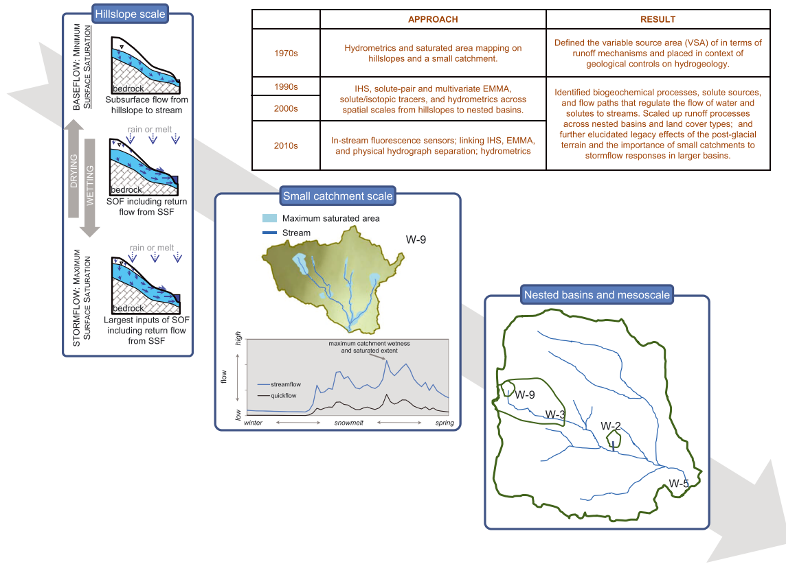
Figure 2. Schematic of flow generation mechanisms and timeline of hydrologic research at Sleepers River Research Watershed
